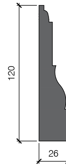
Architrave A1038
