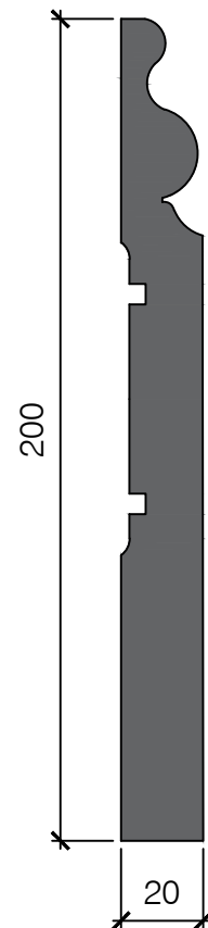
Ogee Skirting S630-1
