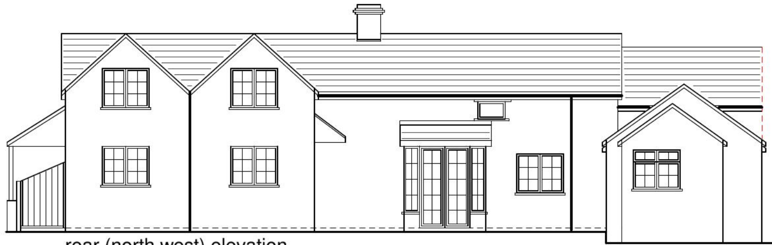
rear (north west) elevation
