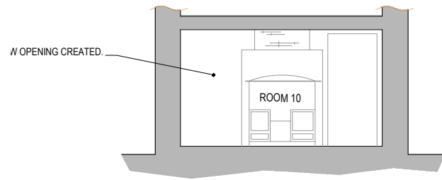
ELEVATION A-A SCALE - 1:50
