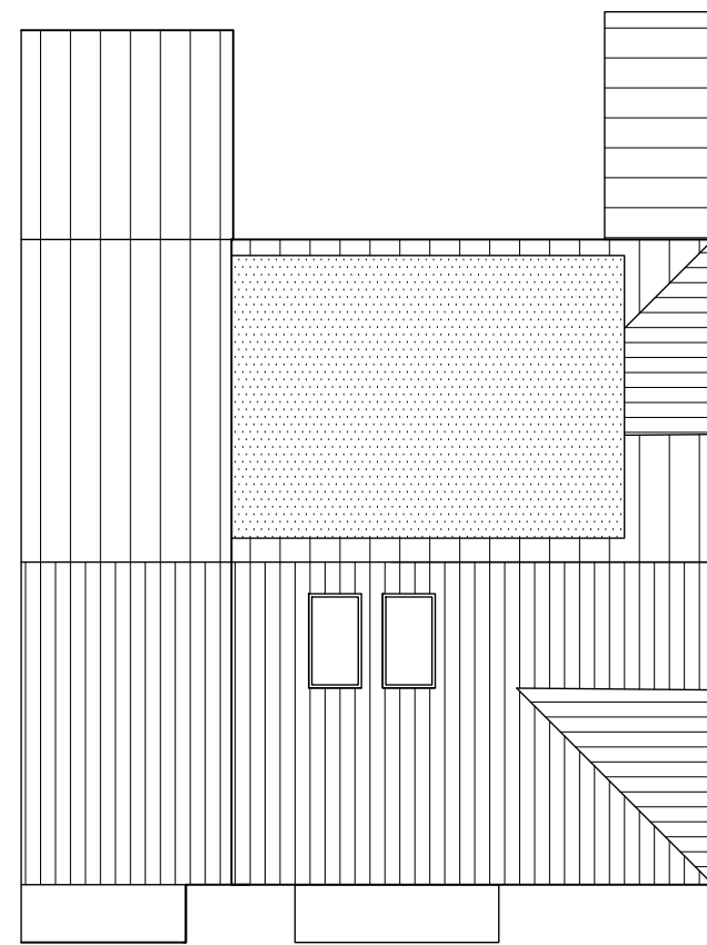
ROOF PLAN
