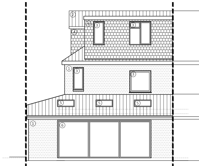
SOUTH WEST ELEVATION - REAR
