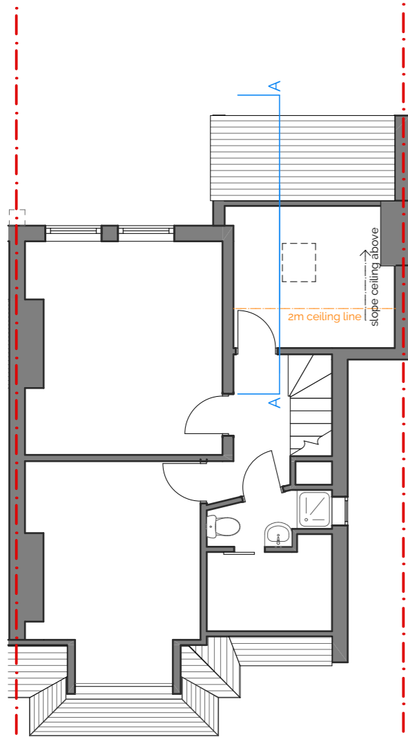
EXISTING SECOND FLOOR PLAN SCALE: 1:100
