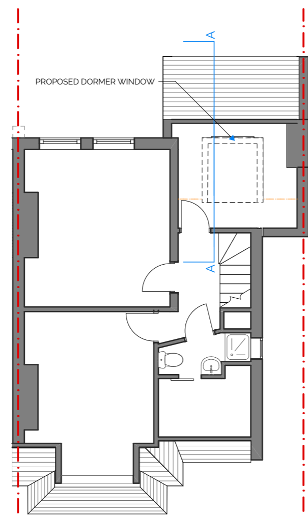
PROPOSED SECOND FLOOR PLAN SCALE: 1:100
