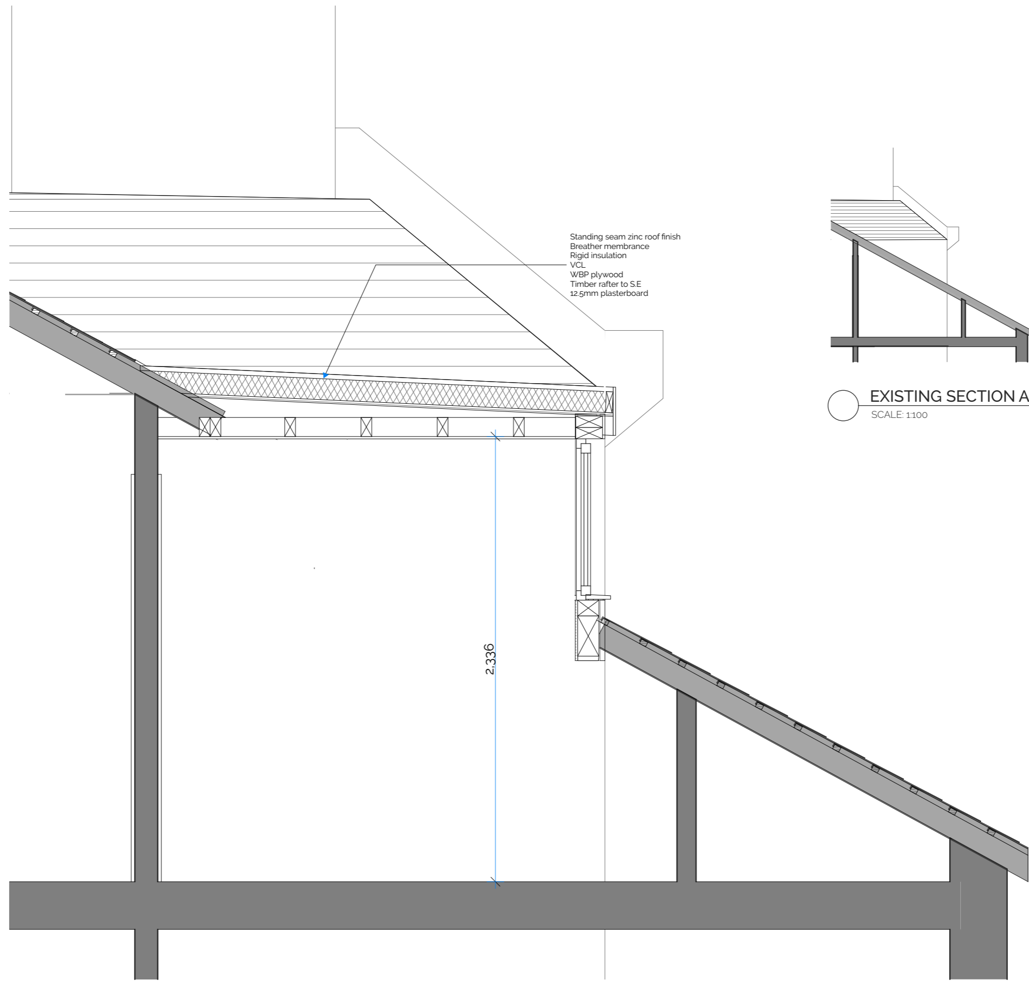
PROPOSED SECTION A SCALE: 1:20
