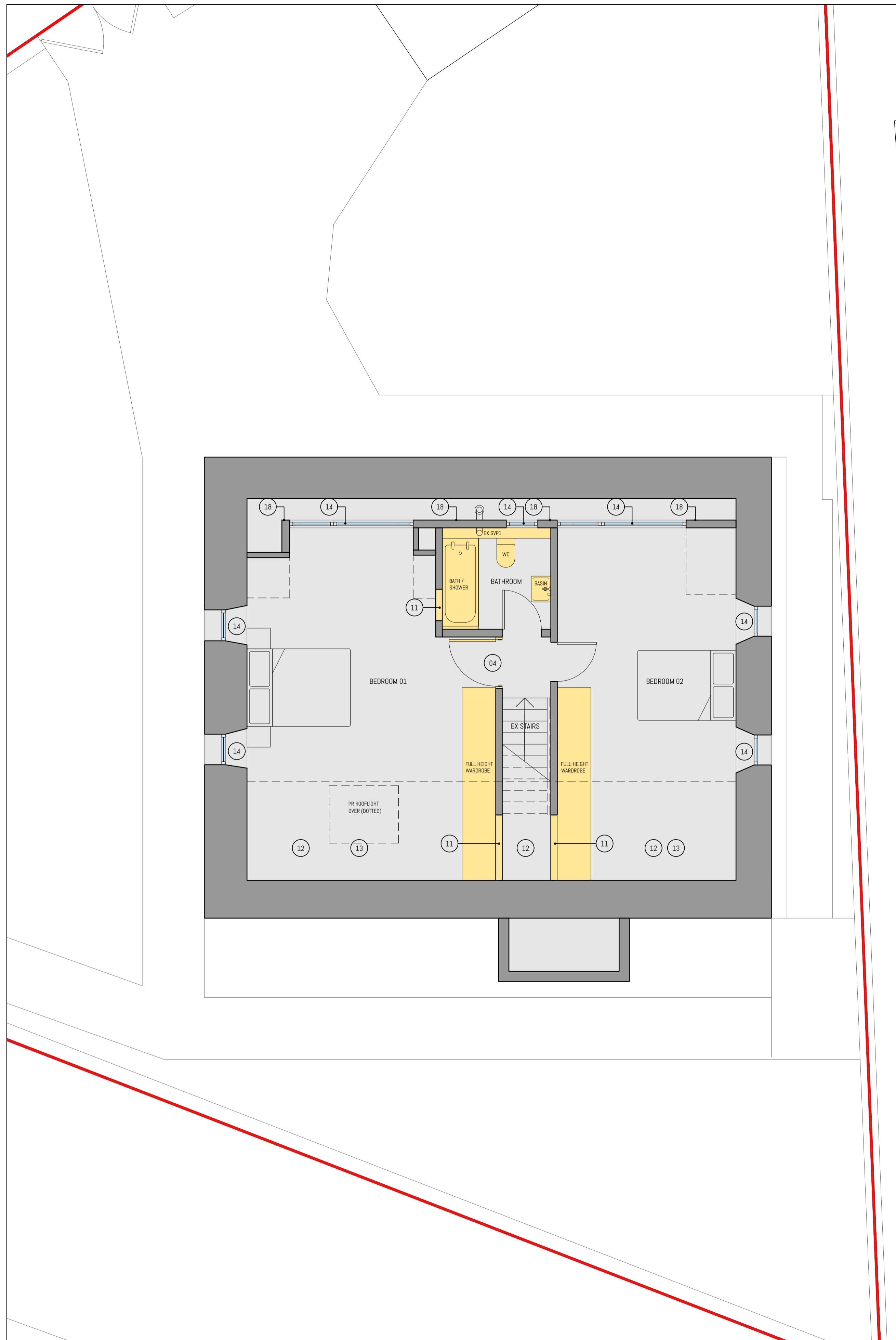
PL-004 2 PROPOSED / PLAN / FIRST FLOOR SCALE 1:50 A1 / 1:100 A3
