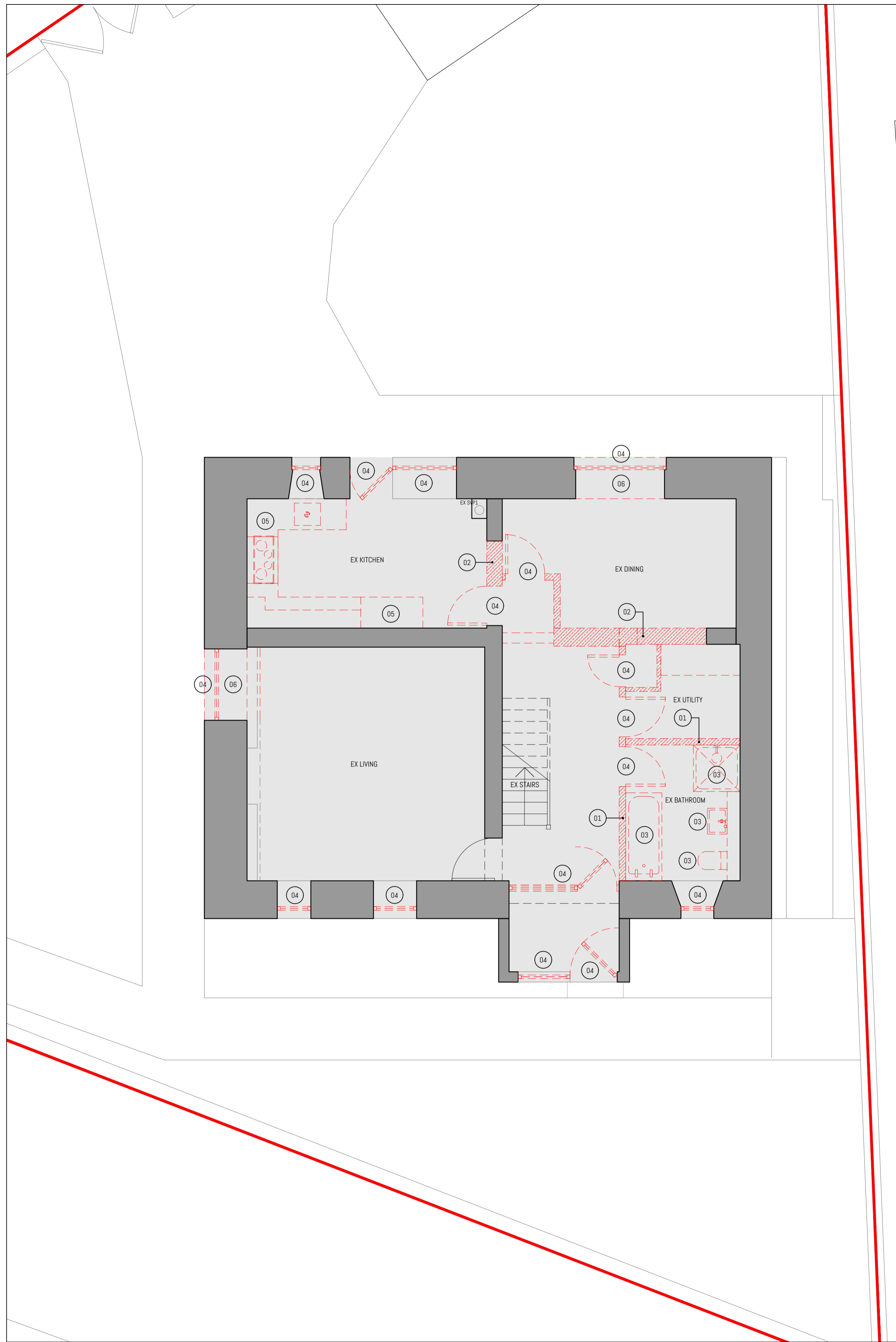
PL-003 1 EXISTING / PLAN / GROUND FLOOR SCALE 1:50 A1 / 1:100 A3
