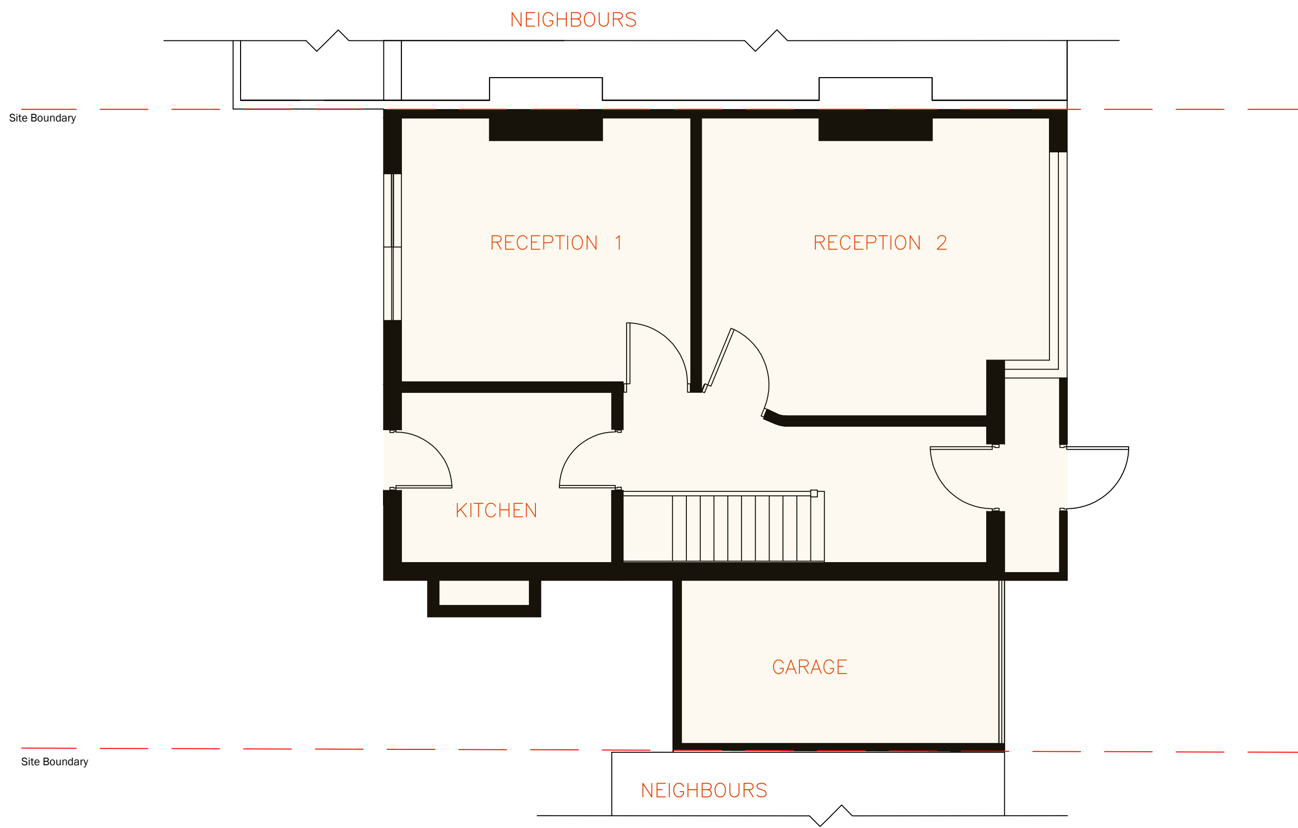
Existing Ground Floor - Plan View
