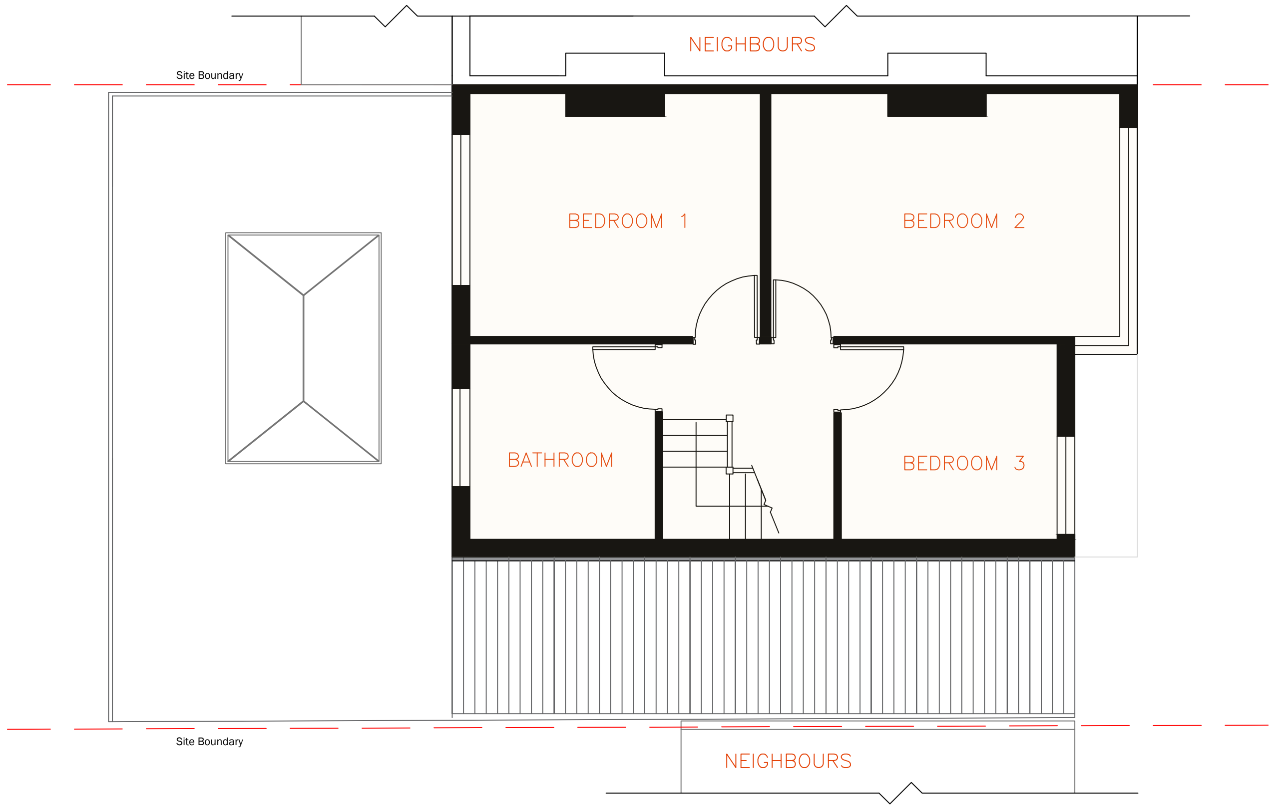
Proposed First Floor - Plan View
