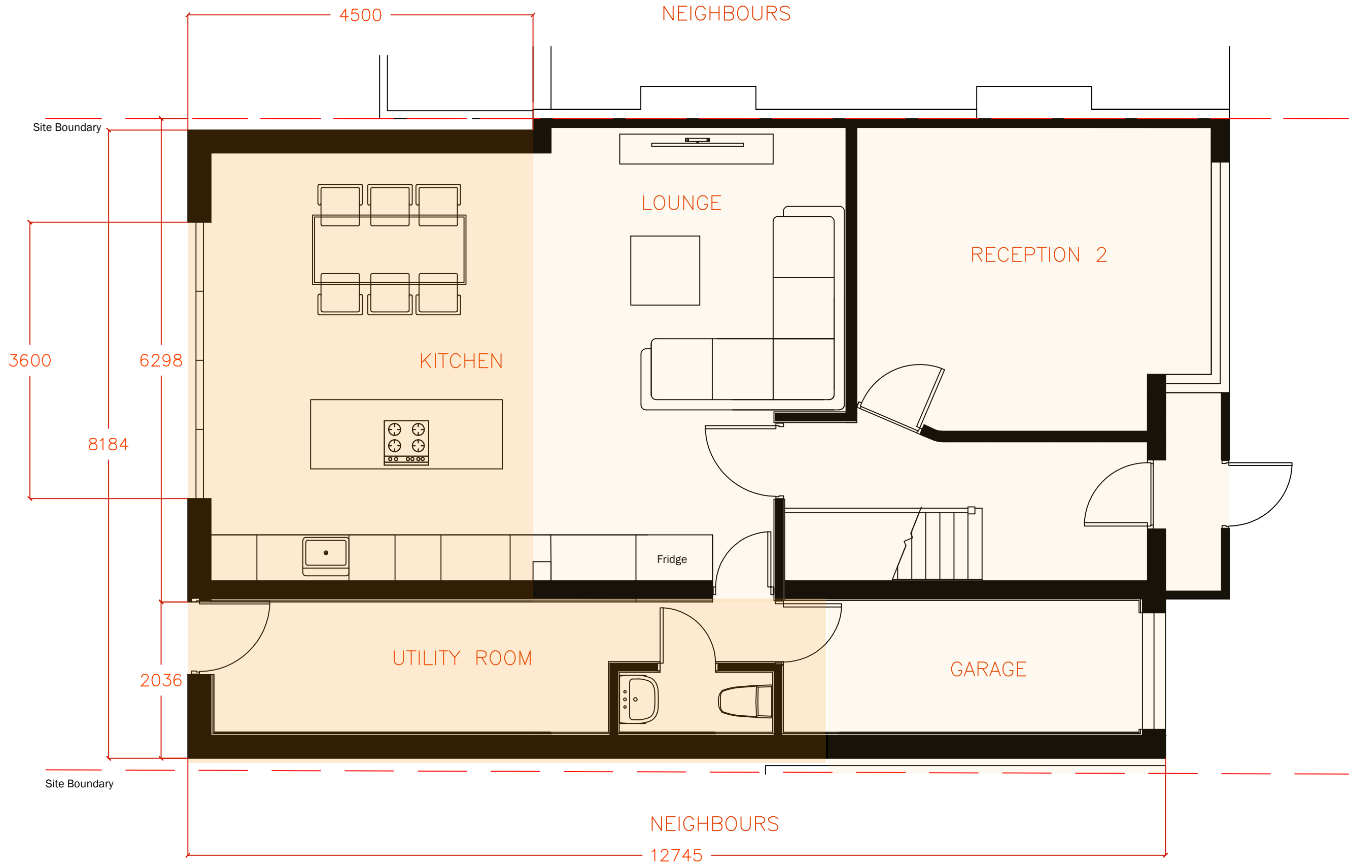
Proposed Ground Floor - Plan View
