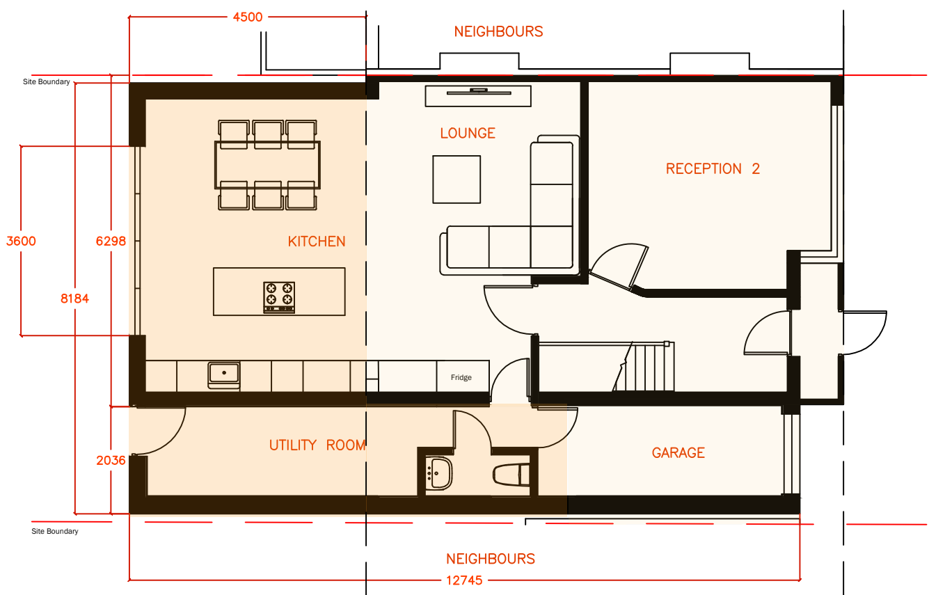
Proposed Ground Floor - Plan View
