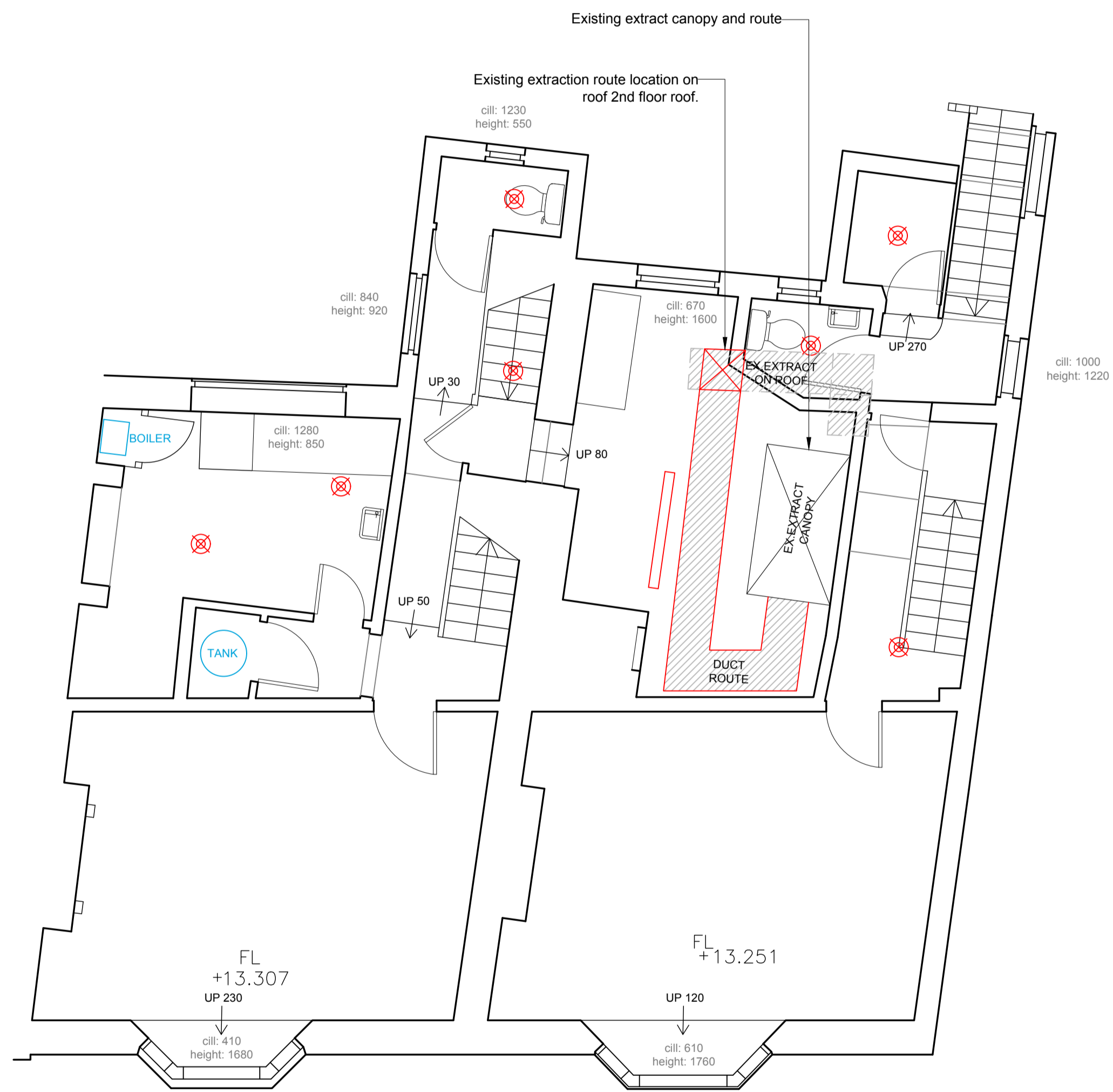
EXISTING FIRST FLOOR LAYOUT
