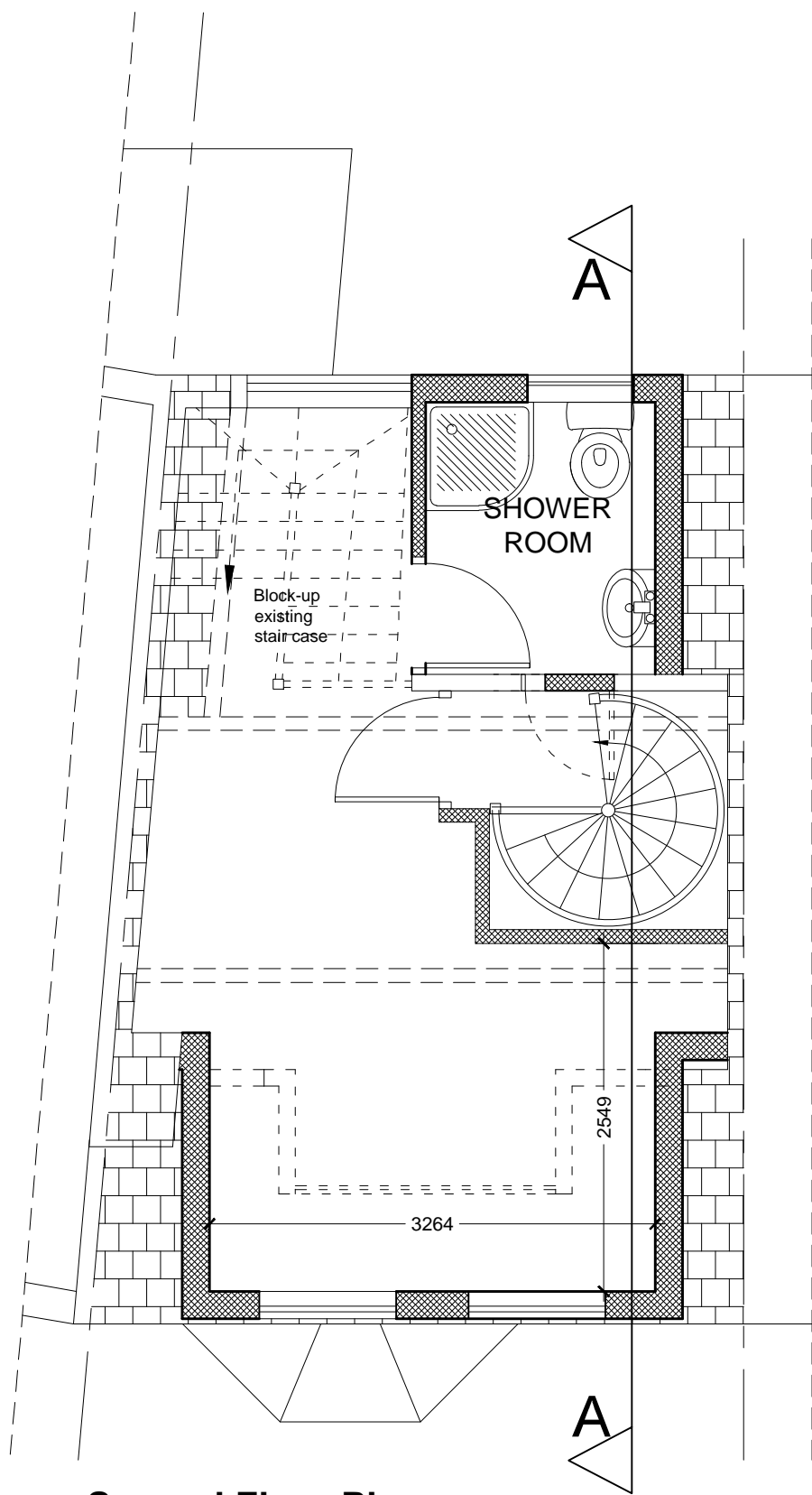
Second Floor Plan Scale 1:50
