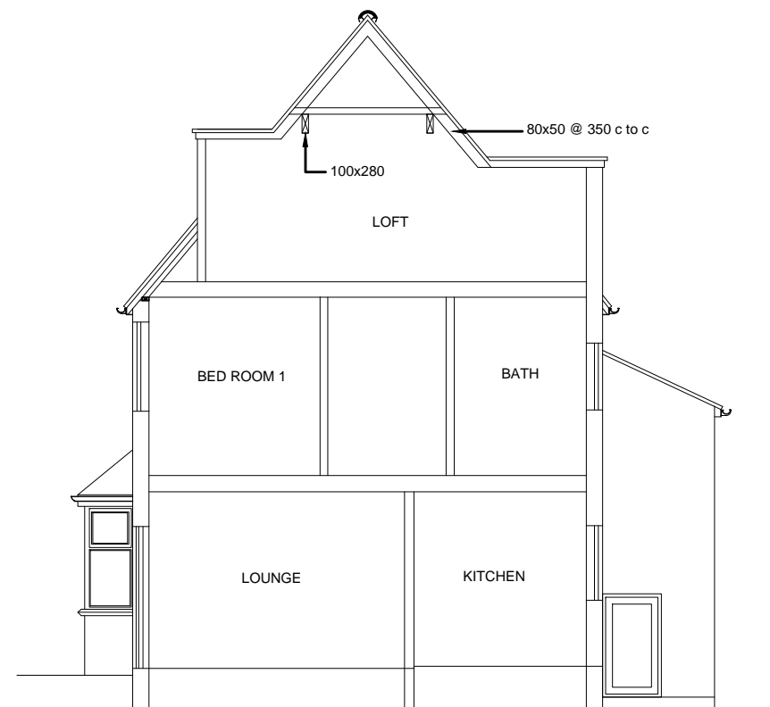
Typical Section Scale 1:100
