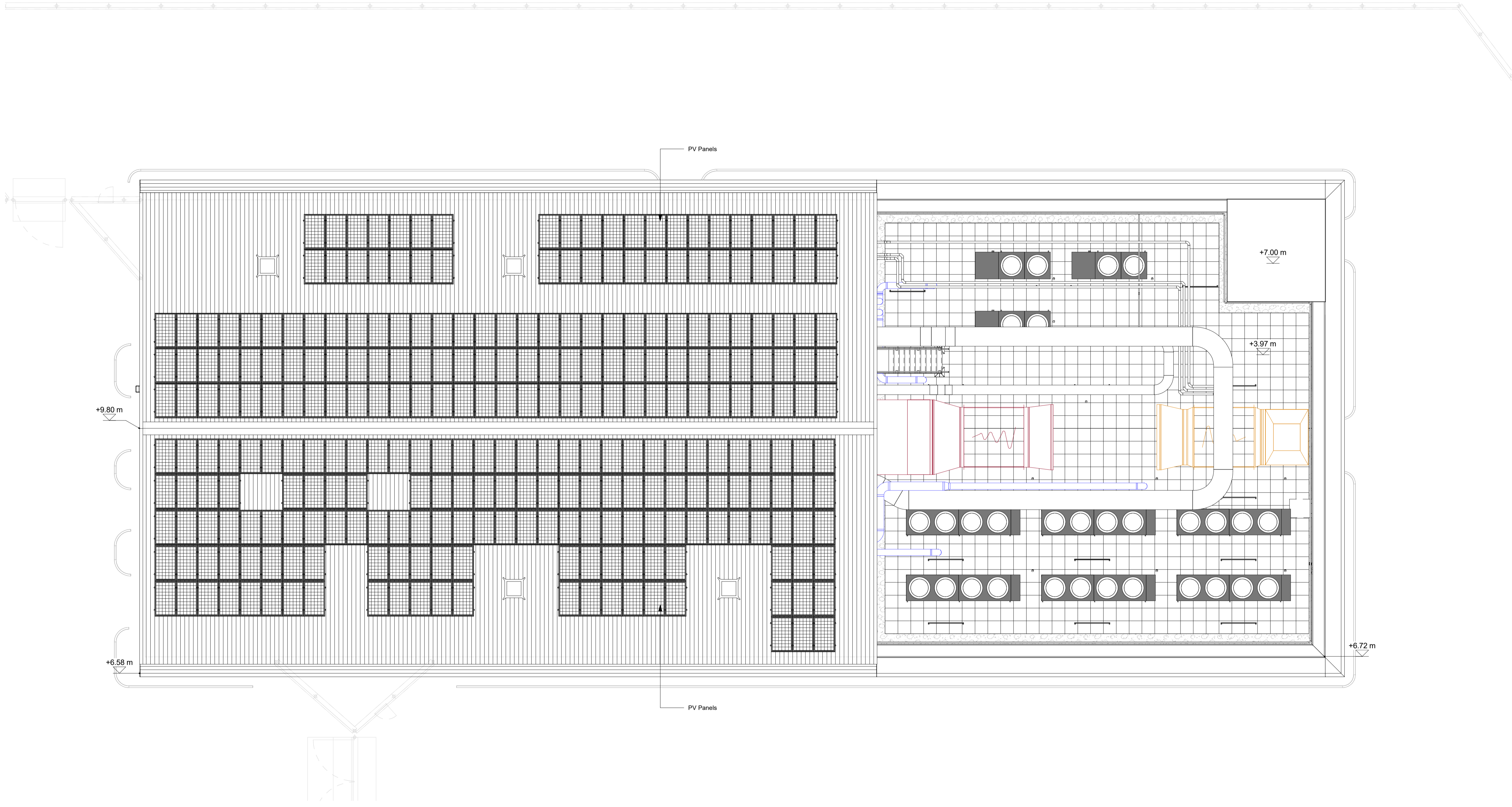
1 Plan-Planning-R01(Roof) 9003 1:100
