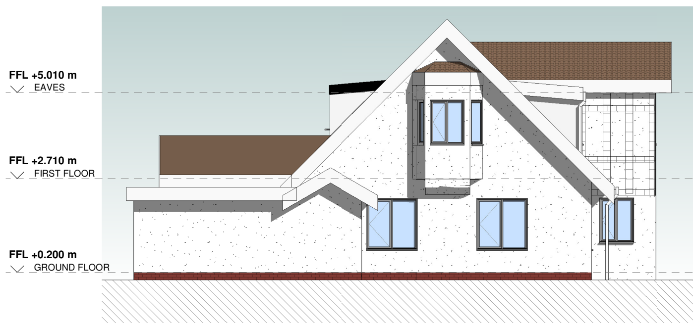
2 WEST ELEVATION - EXISTING 1 : 100
