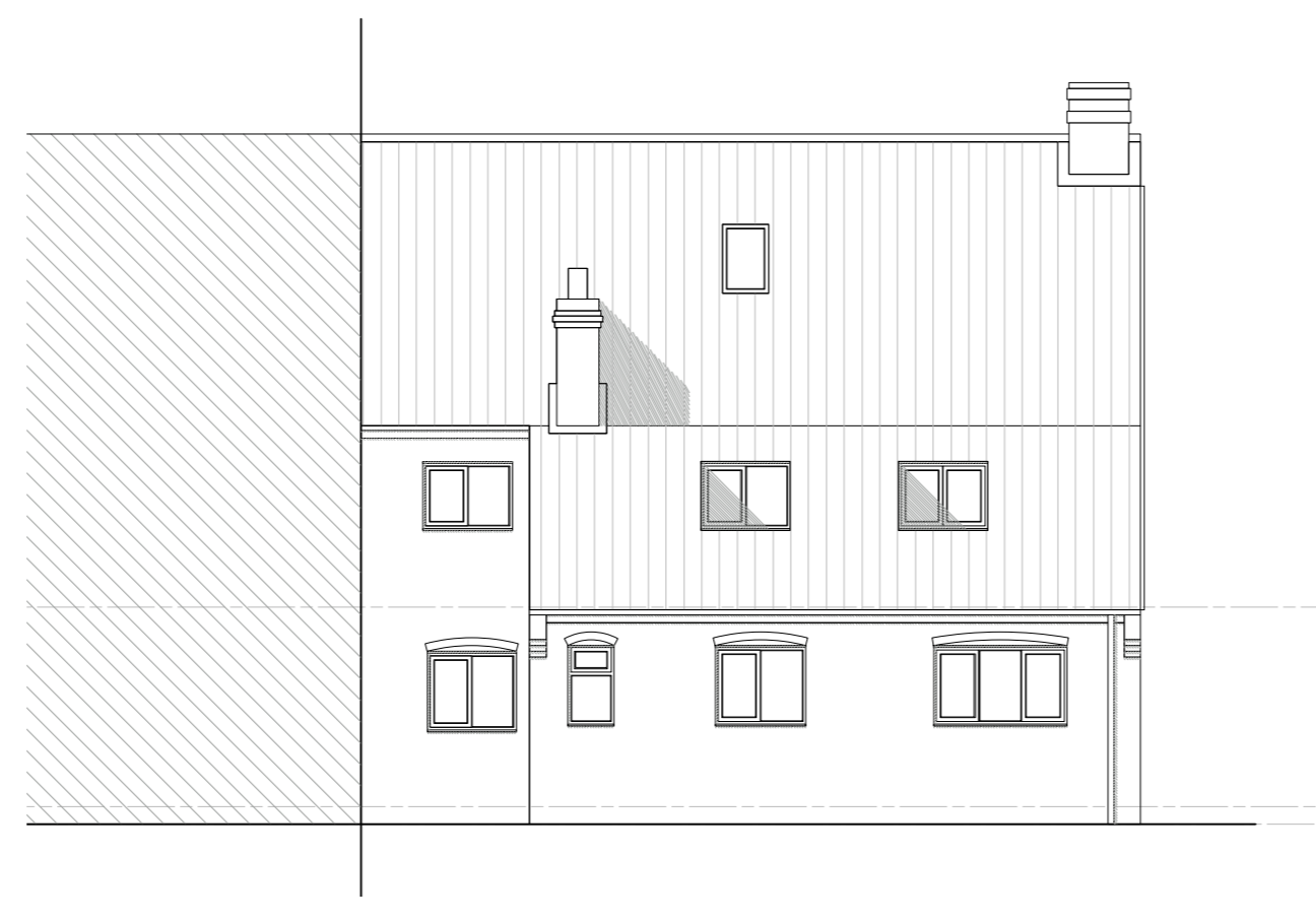
6 REAR ELEVATION 1:100 @ A1
