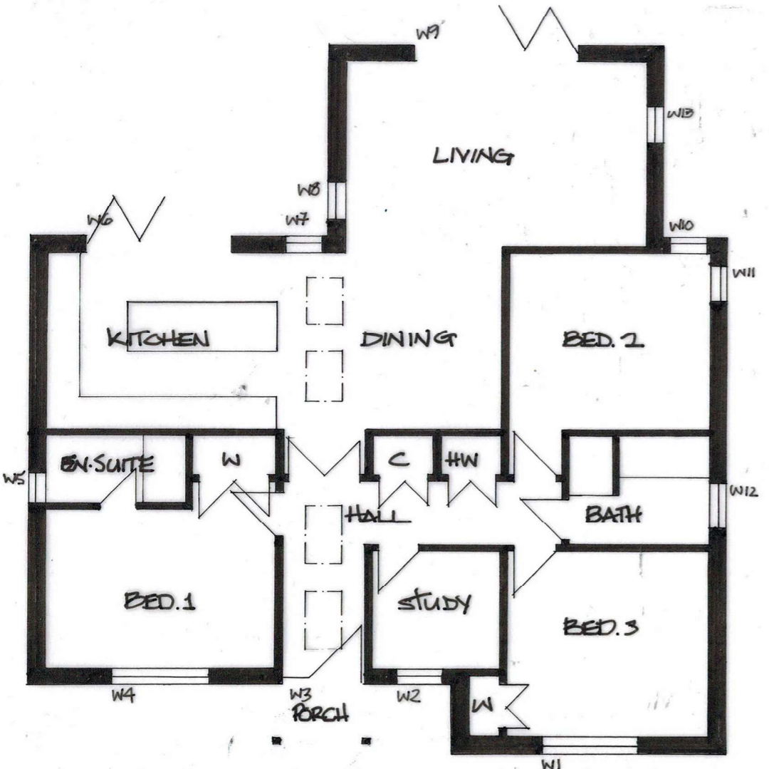
FLOOR PLAN
