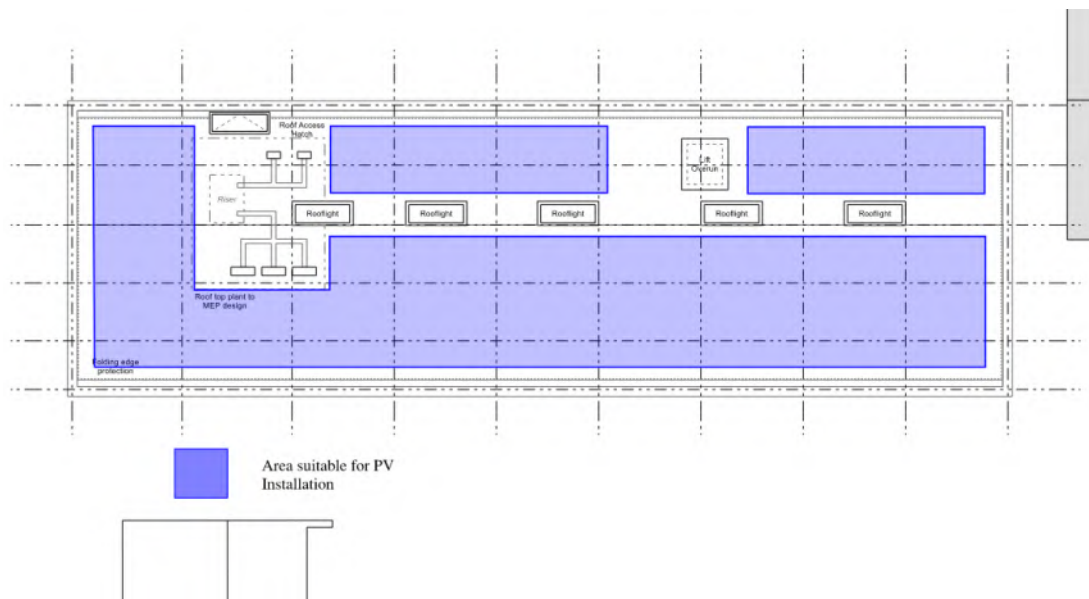
Figure 4.1: Potential PV panels positions on flat roofs
