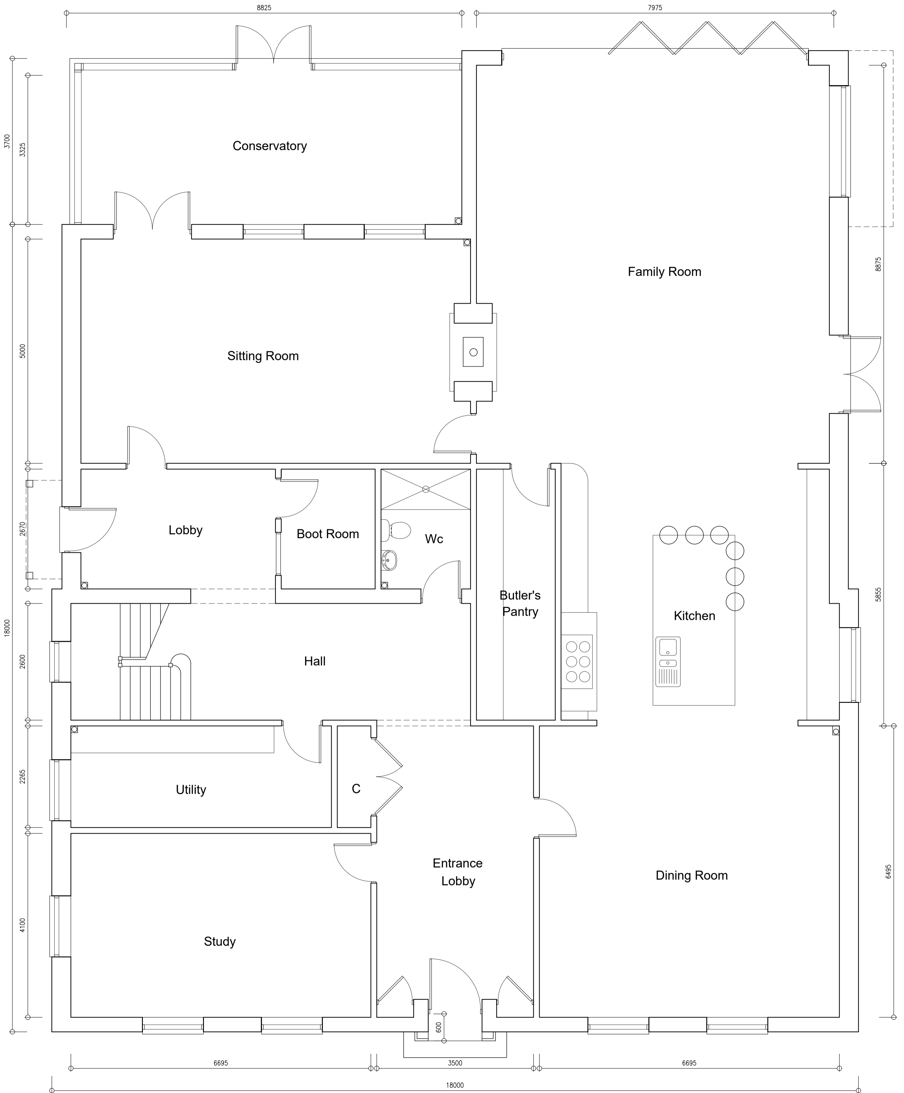
Proposed Ground Floor Plan 1:50
