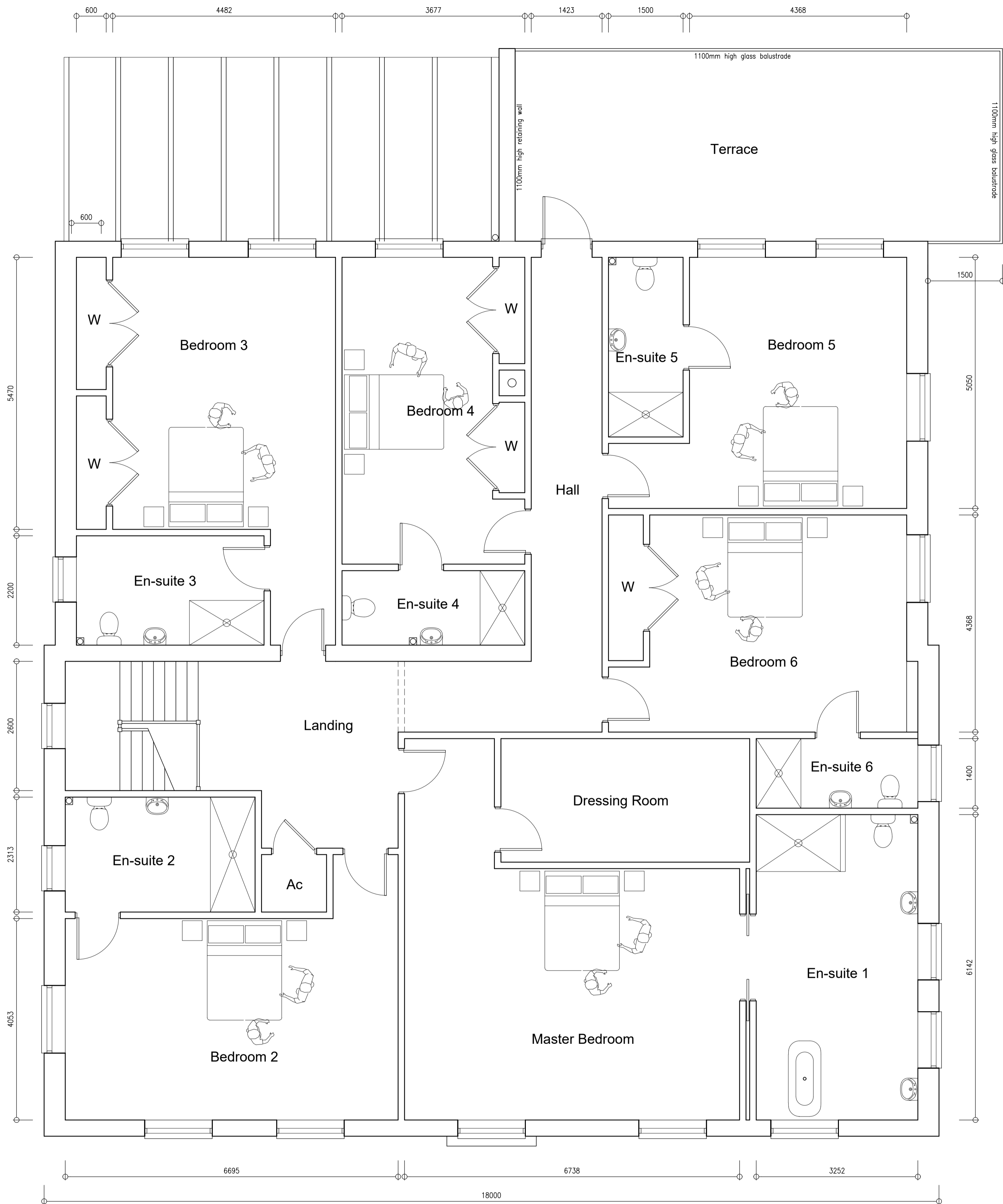
Proposed First Floor Plan 1:50
