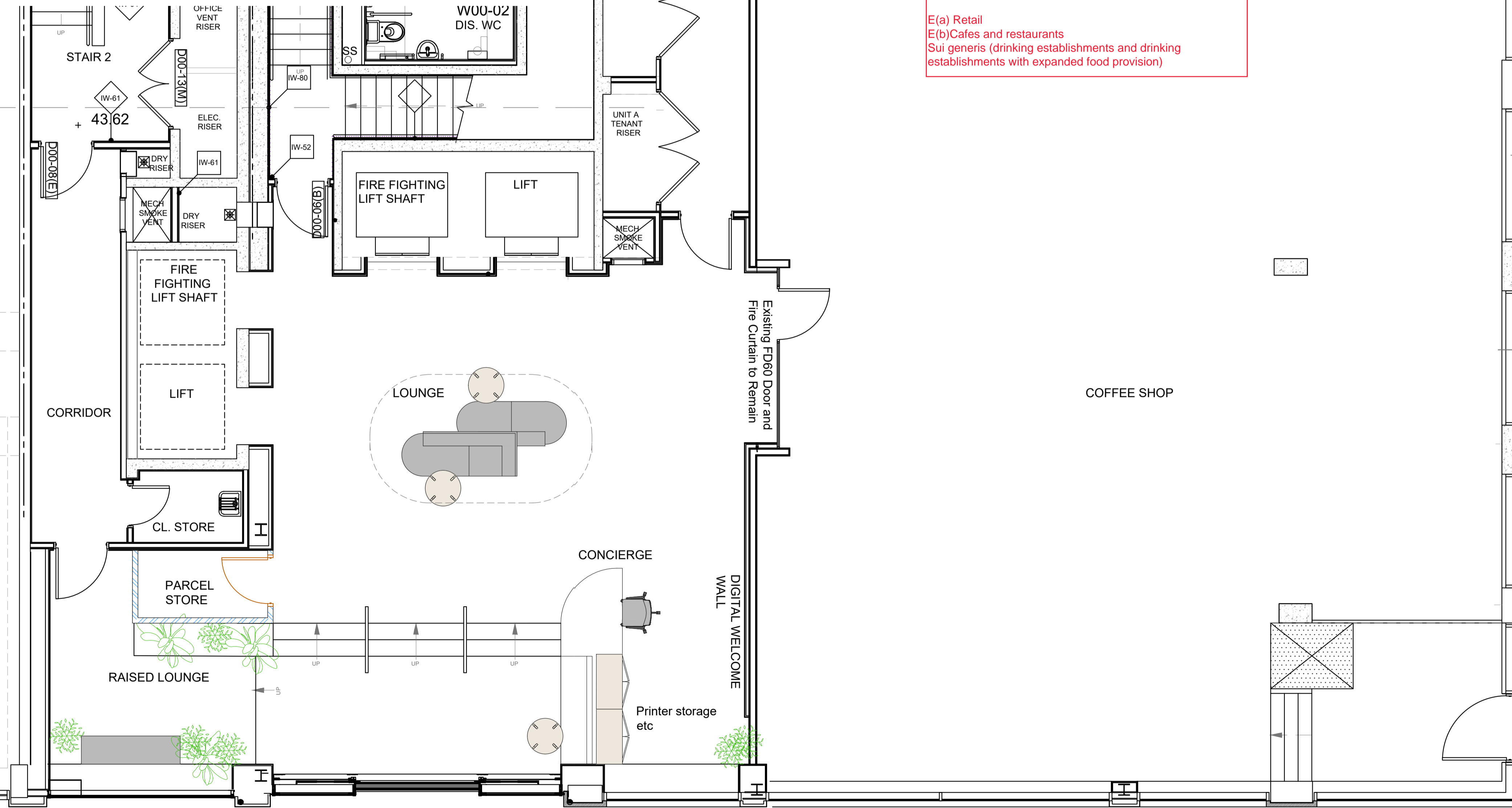
GROUND FLOOR @1:50
