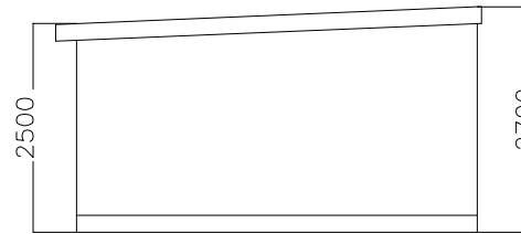
OUTBUILDING SIDE ELEVATION
