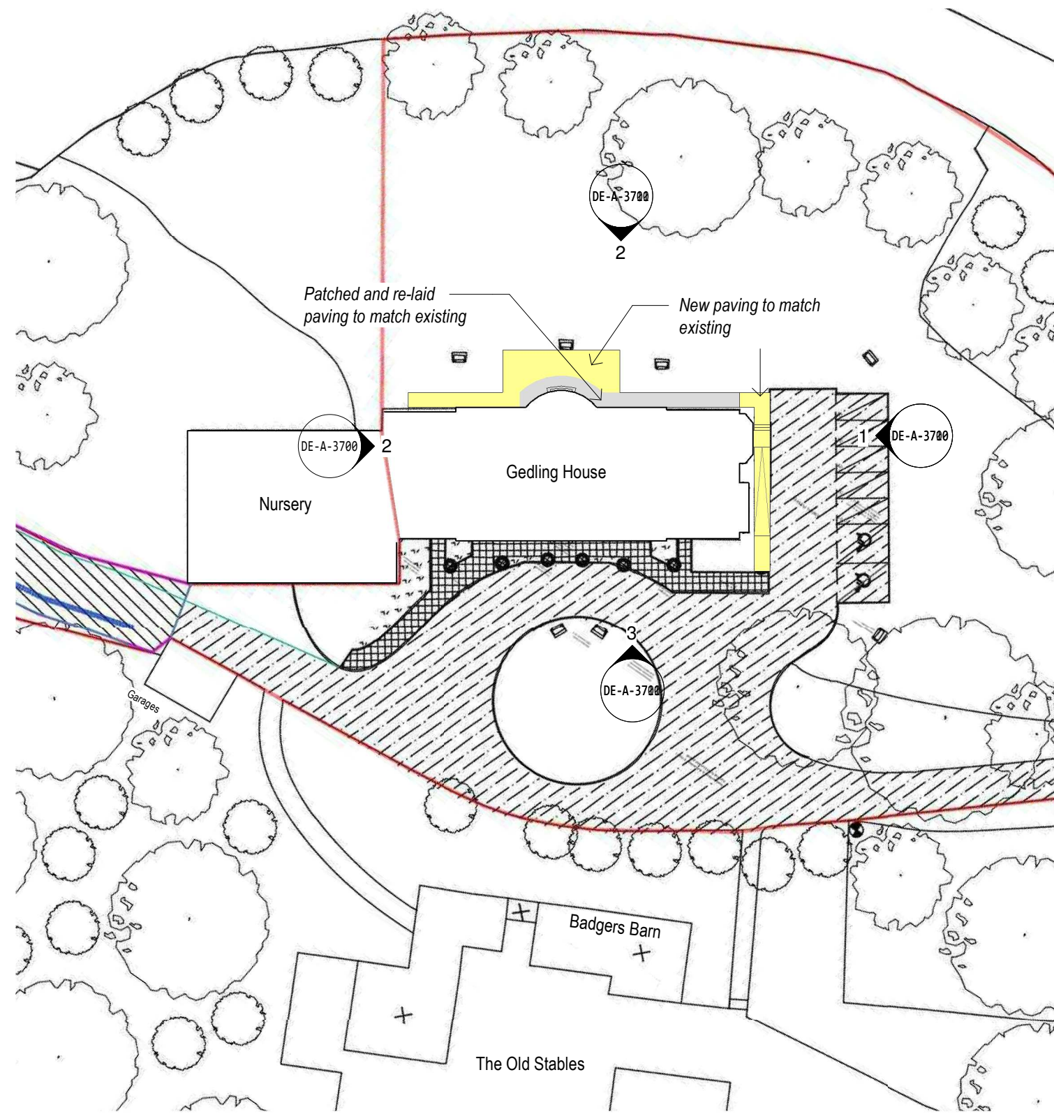
1 Proposed Site Plan 1 : 500
