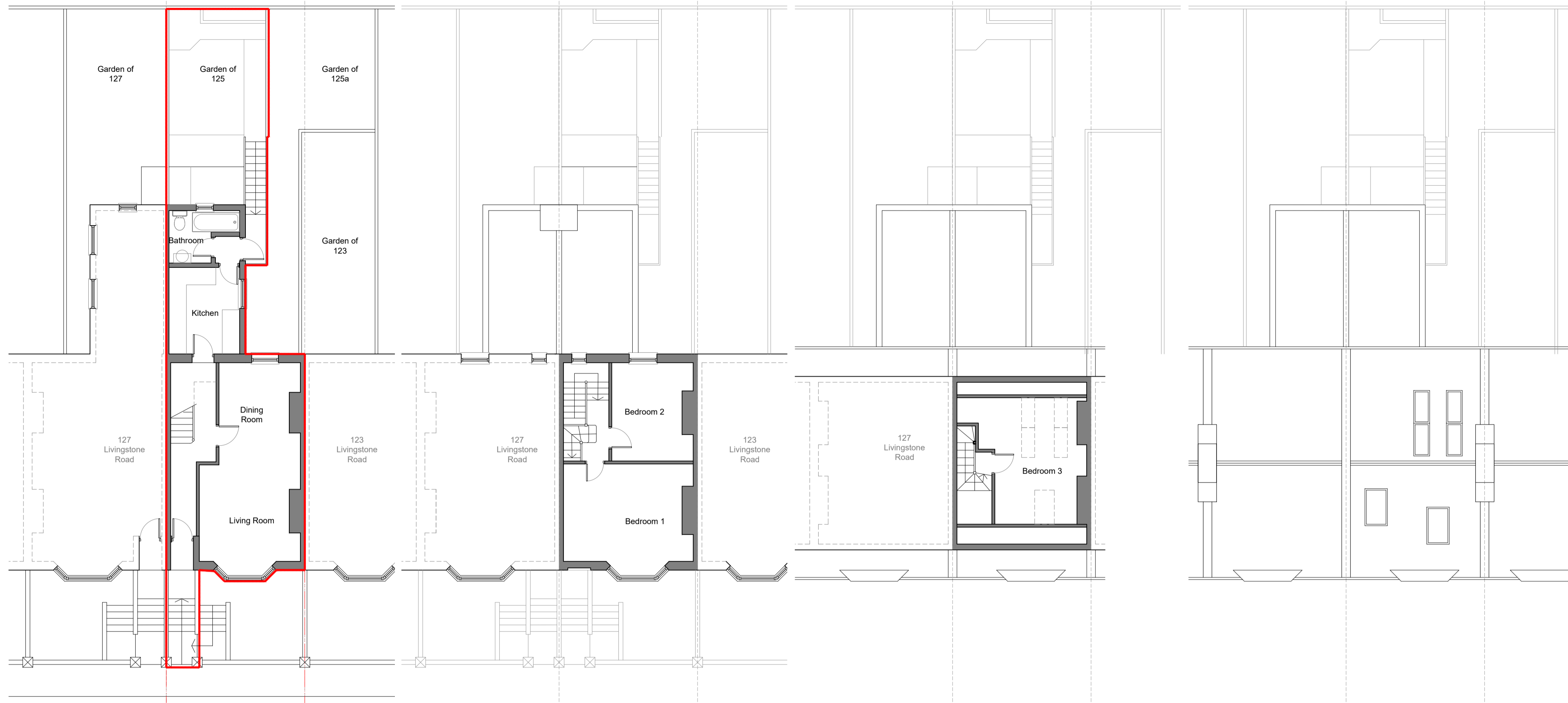
01 Ground Floor Plan Scale:1:100
