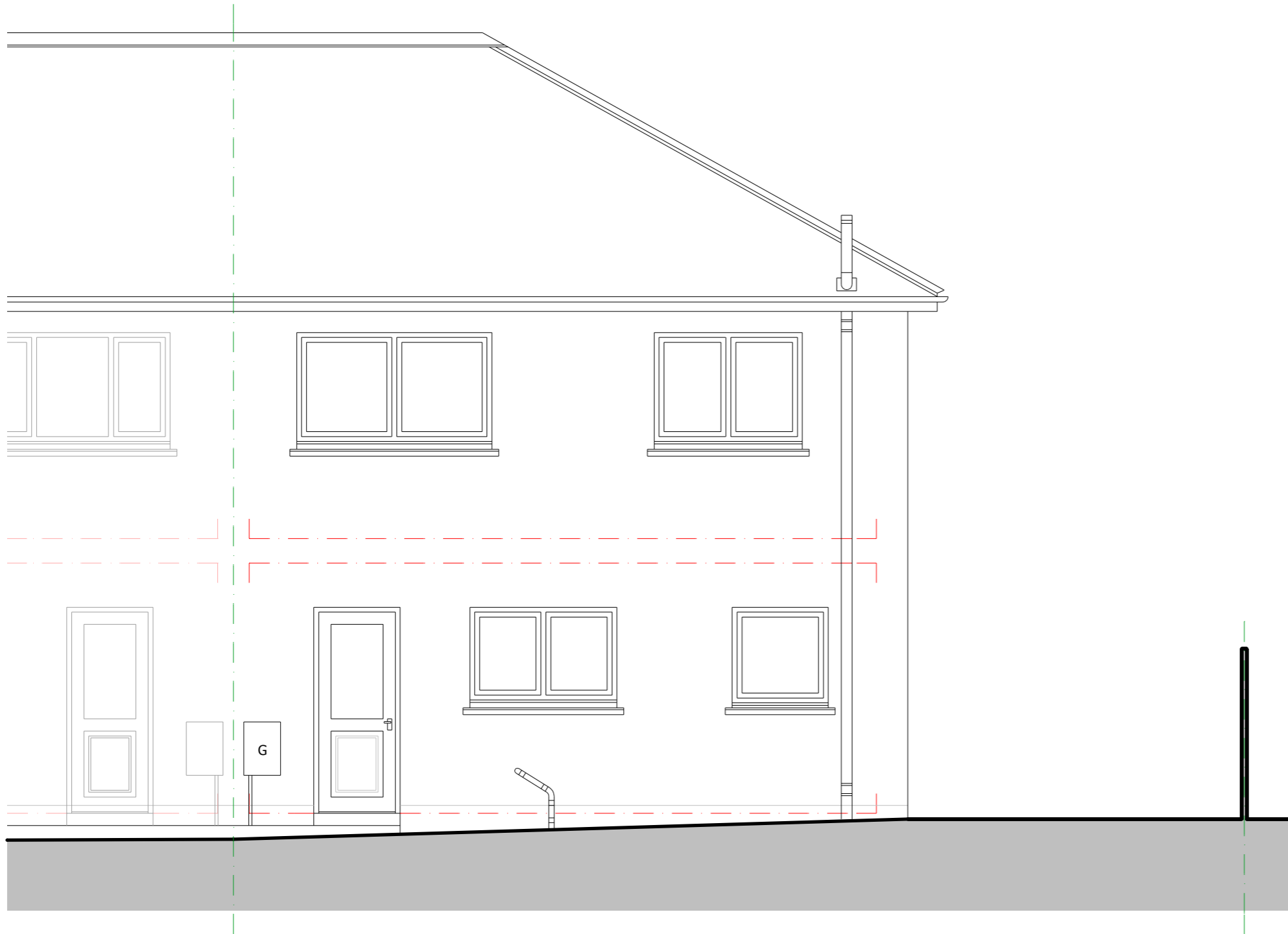
NORTH ELEVATION :
