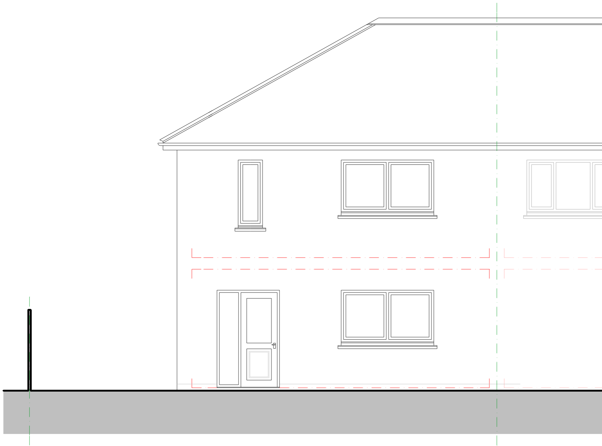
SOUTH ELEVATION :
