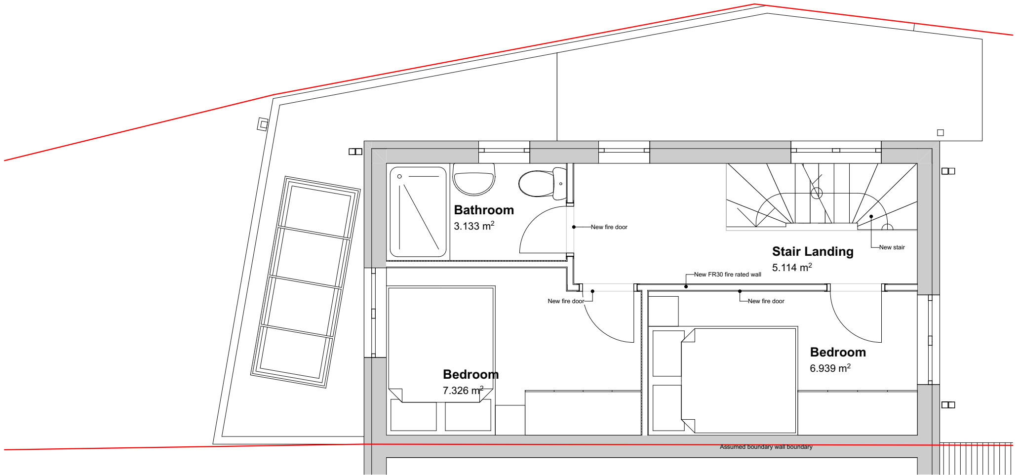
16 Hoddesdon Rd, Belvedere Proposed First Floor Plan 1:50
