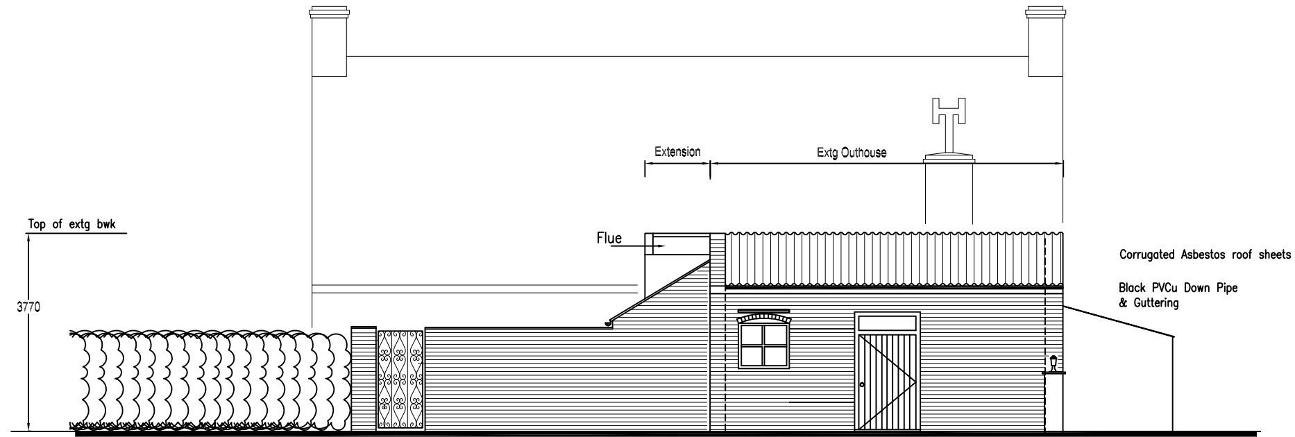
North Elevation
