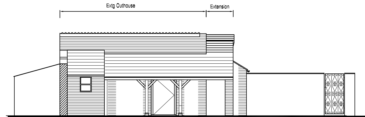
South Elevation (Courttyard Elevation)
