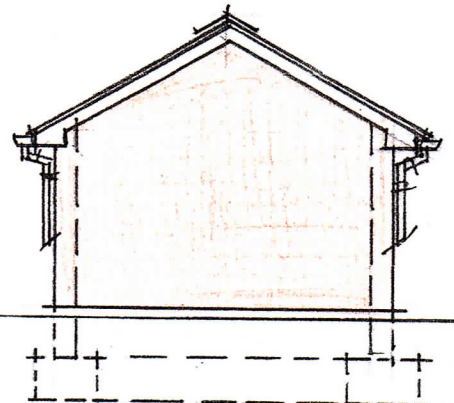
WEST ELEV. 1:100
