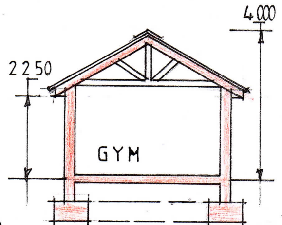
TYPICAL SECTION
