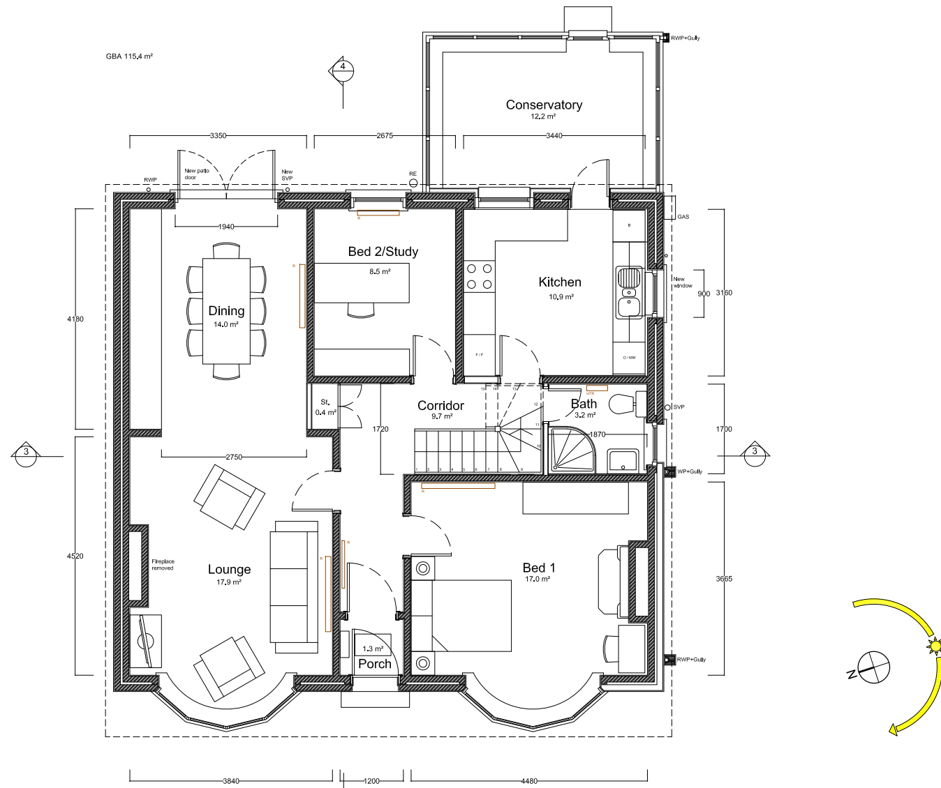
1 Ground Floor Plan 1:100 @ A3
