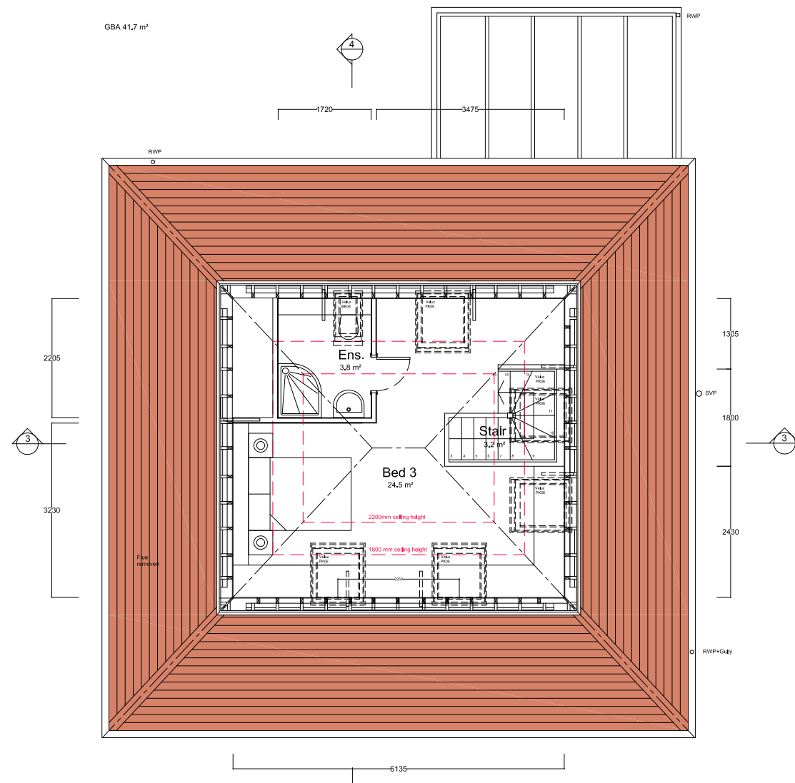
2 First Floor Plan 1:100 @ A3
