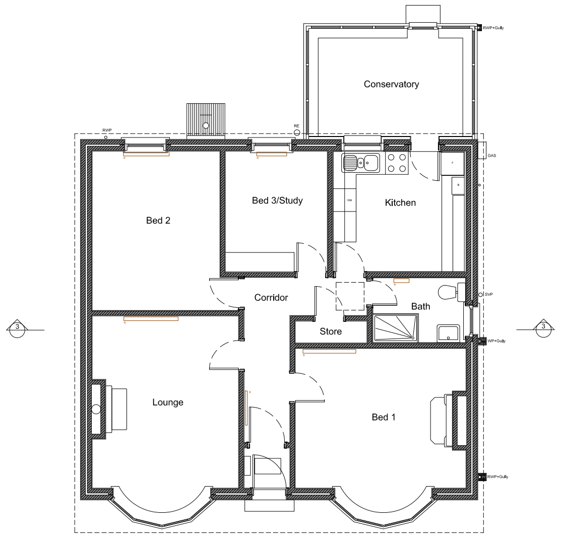
1 Ground Floor Plan 1:100 @ A3
