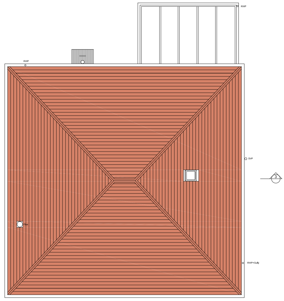
2 Roof Plan 1:100 @ A3
