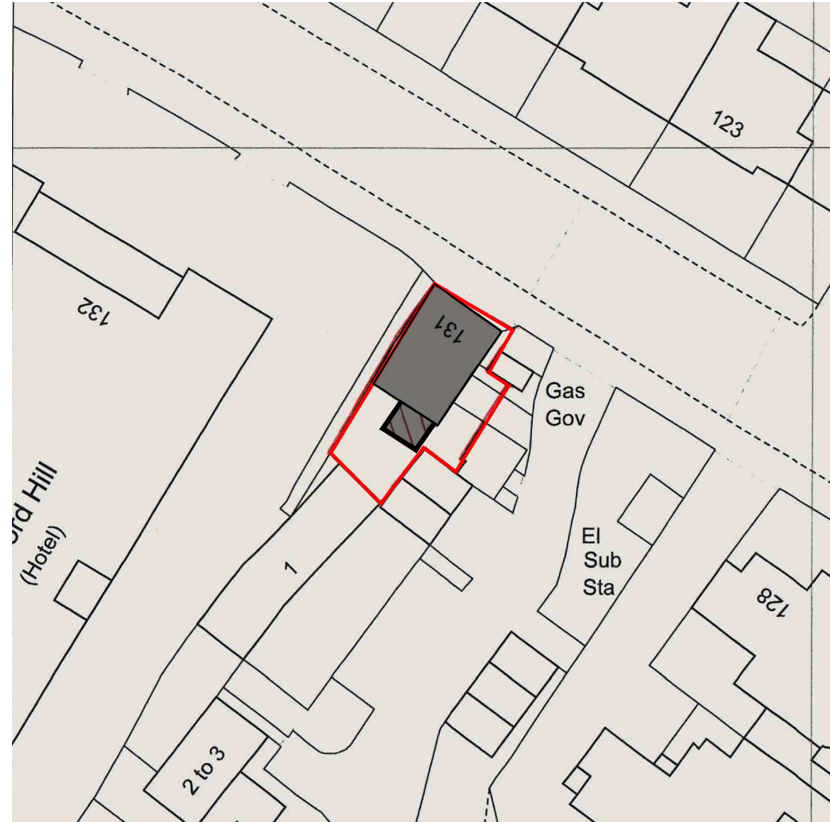
BLOCK PLAN 1:500
