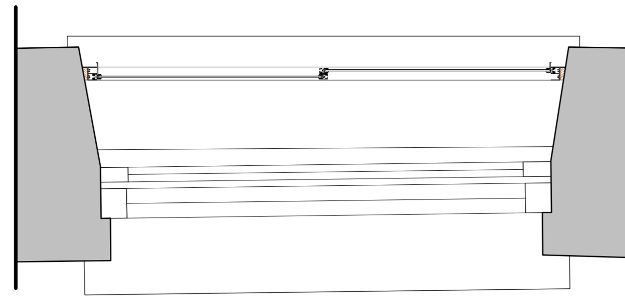
Secondary Glazing Detail 1:10
