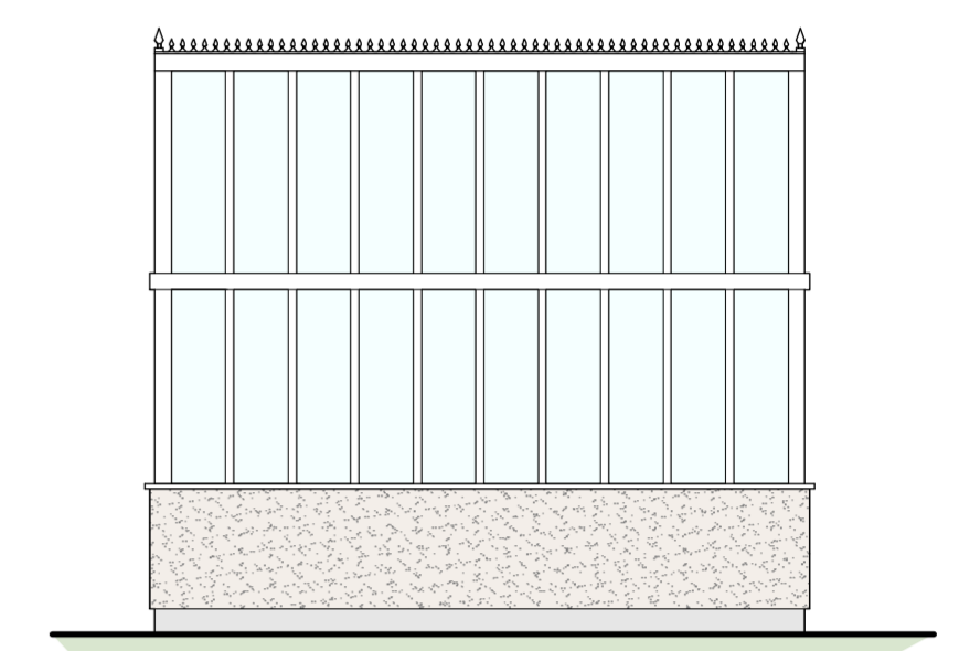
Side Elevation 1:50
