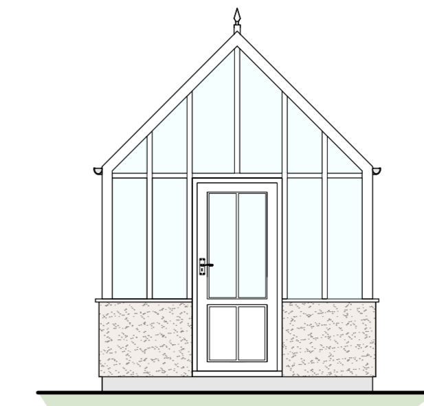
Front Elevation 1:50
