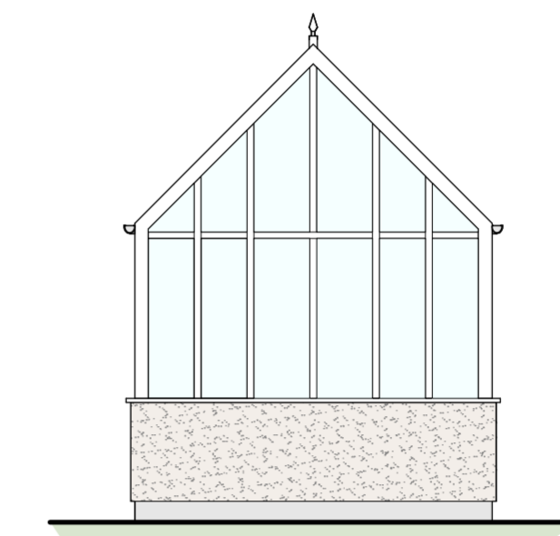
Rear Elevation 1:50
