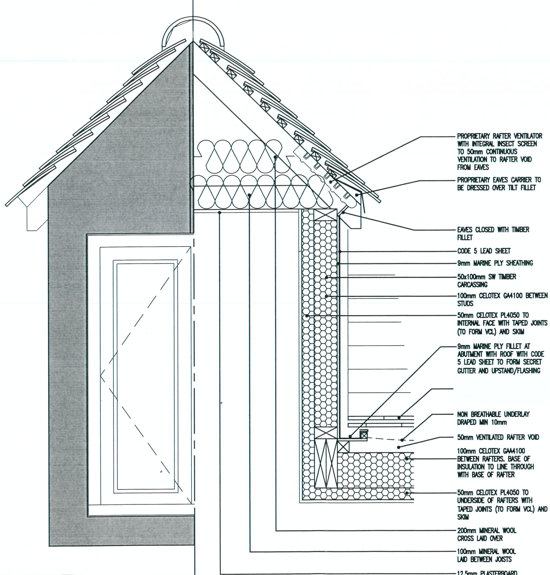
Dormer window detail Scale 1:10 at A3
