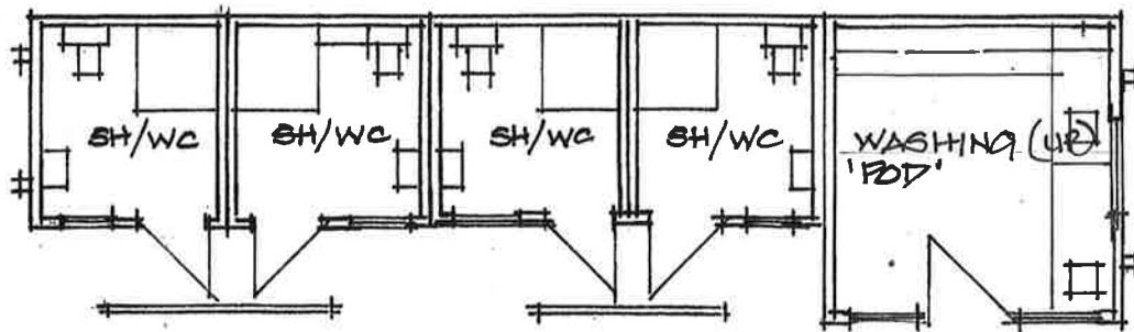
FLOOR PLAN 1:100
