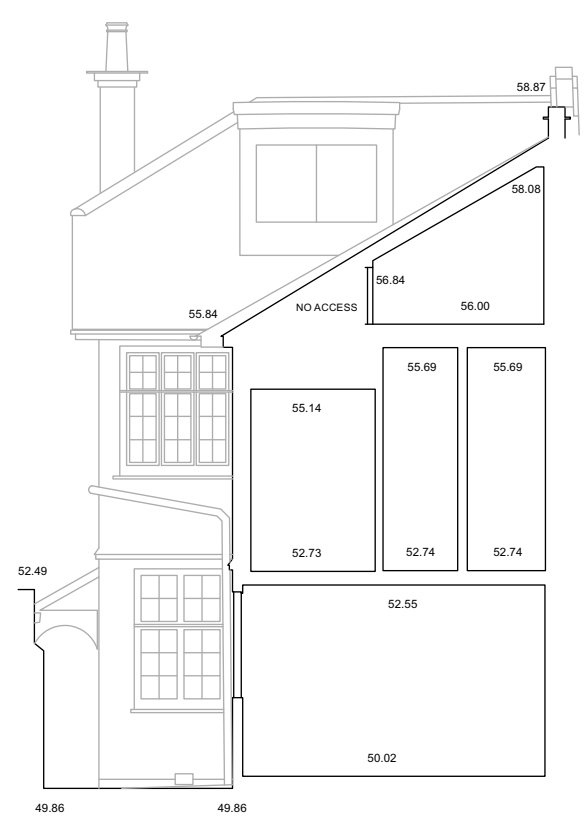
2 Proposed Section DD - No change Scale: 1:100
