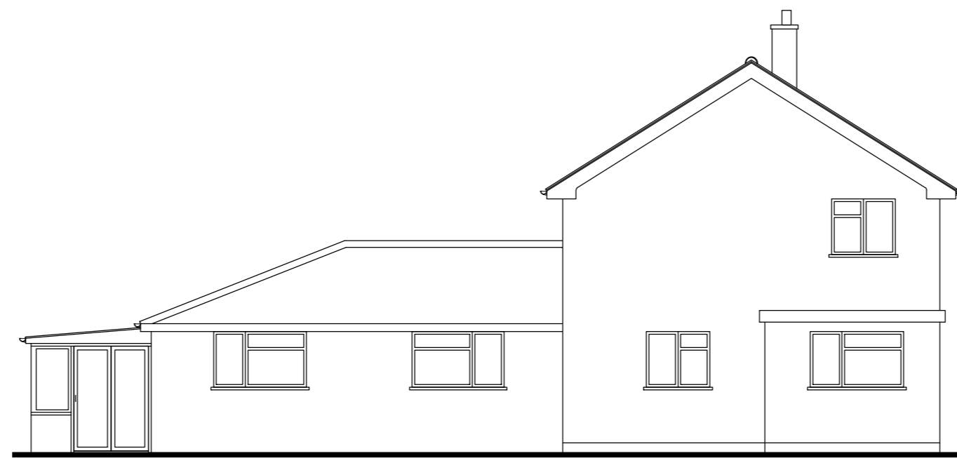
SOUTH ELEVATION
