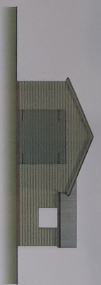
SOUTH EAST ELEVATION SCALE 1:100
