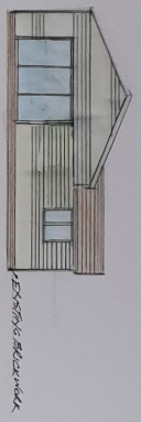
SOUTH EAST ELEVATION SCALE 1:100
