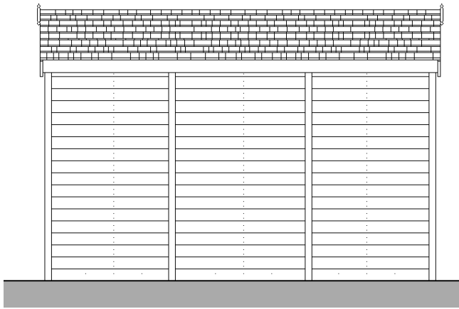
NORTH ELEVATION 1:100 PROPOSED
