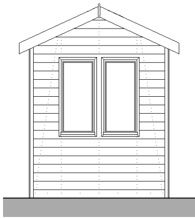
WEST ELEVATION 1:100 PROPOSED
