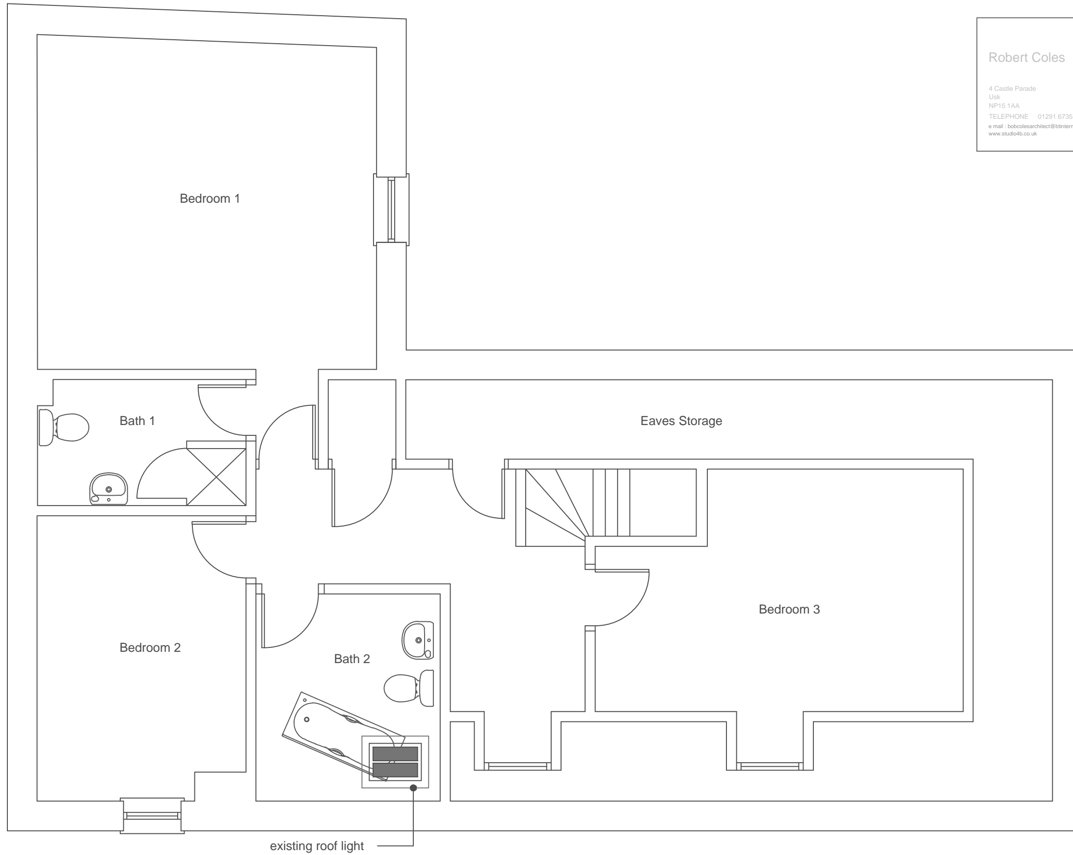
EXISTING PART FIRST FLOOR PLAN 5 DENBURY MEWS USK DRAWING PL02 22July21 Scale 1:50 @ A3
