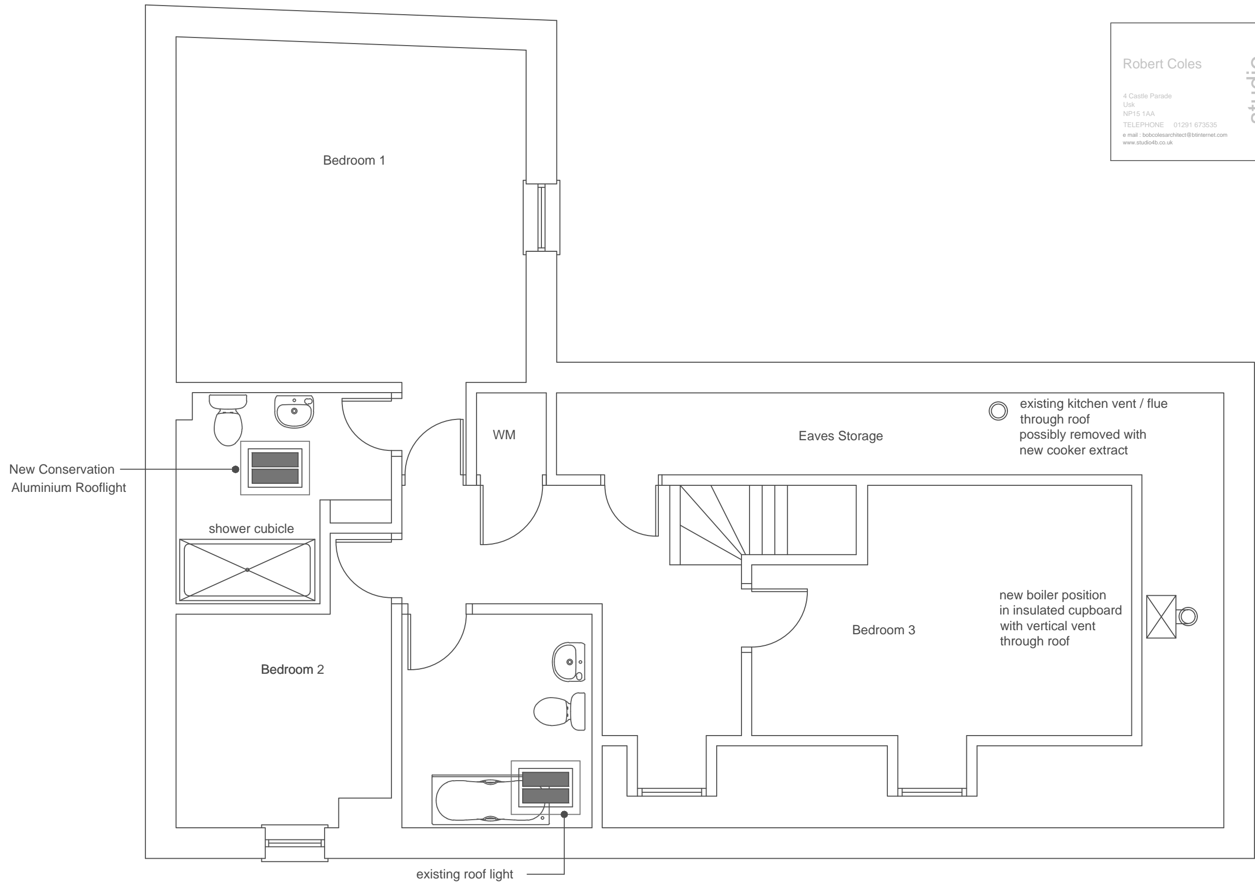
PROPOSED PART FIRST FLOOR PLAN 5 DENBURY MEWS USK DRAWING PL04 2September21 Scale 1:50 @ A3
