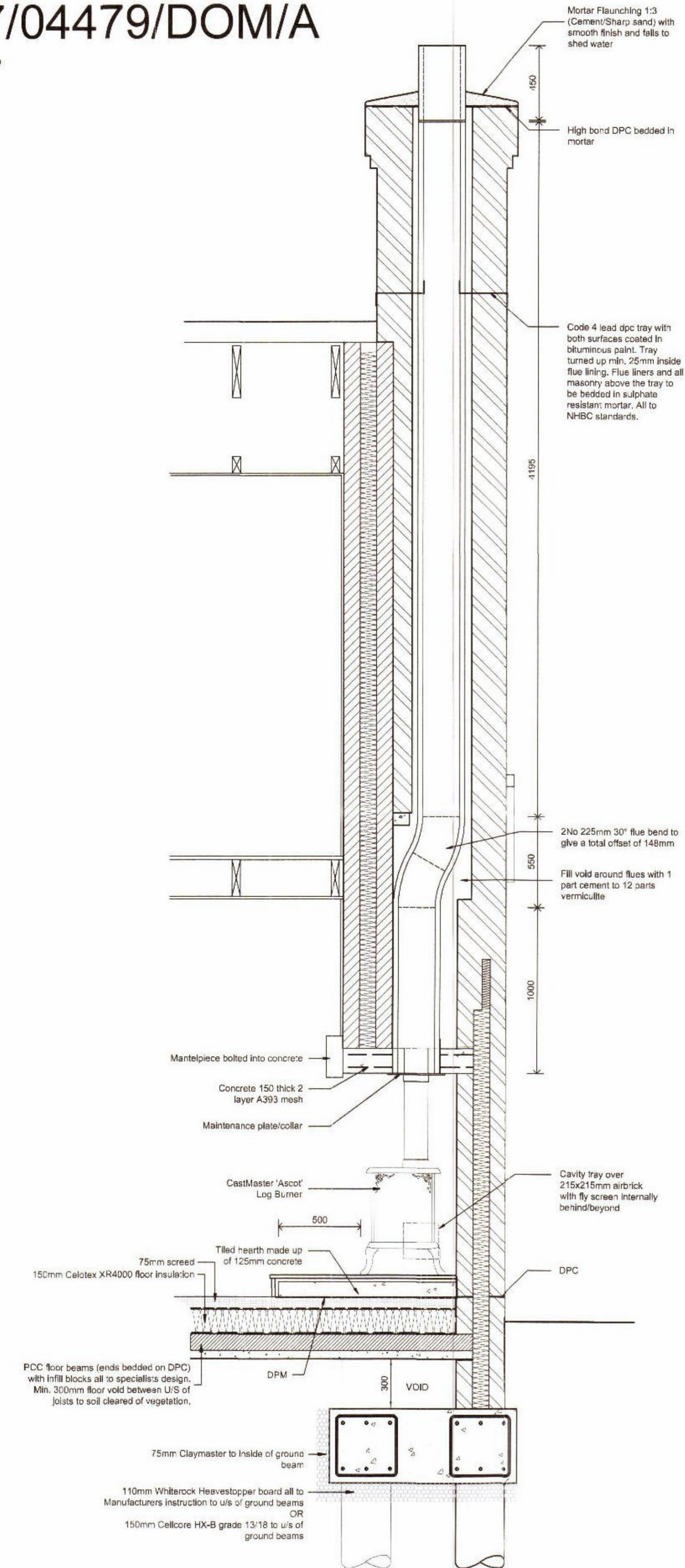
Section E-E Scale 1:20
