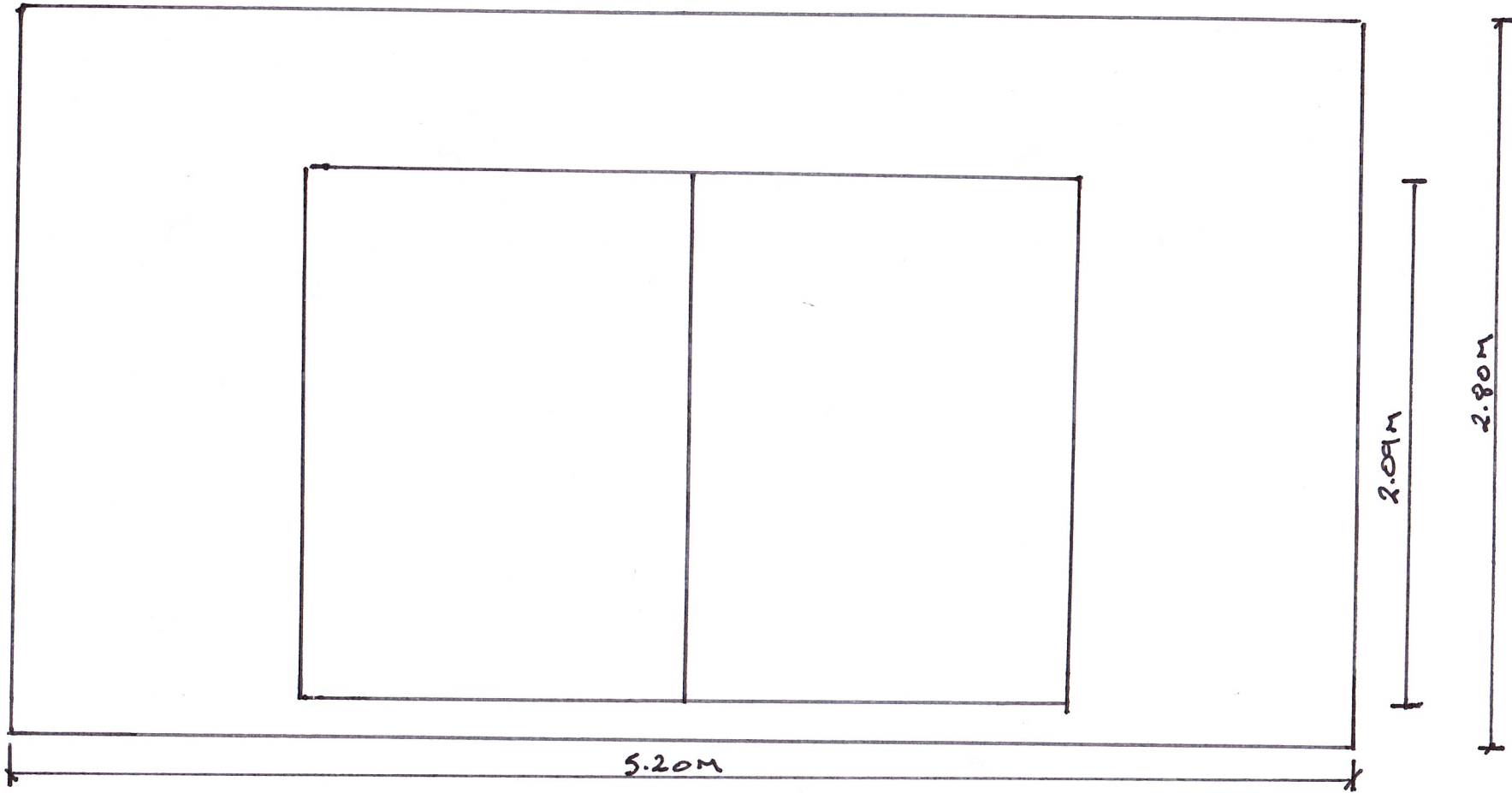
LEAMOUNT : OUTBUILDING FRONT ELEVATION 1:25
