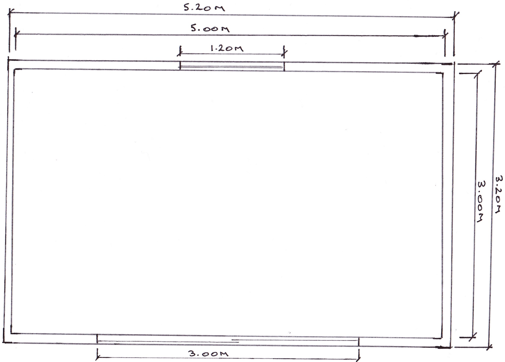
LEAMOUNT: OUTBUILDING FLOOR PLAN 1:25
