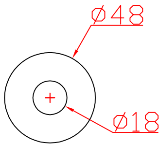
Form "F" Washer 4mm Thick
