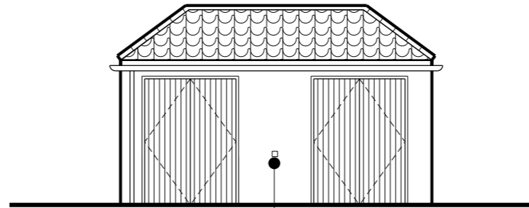
EAST ELEVATION
